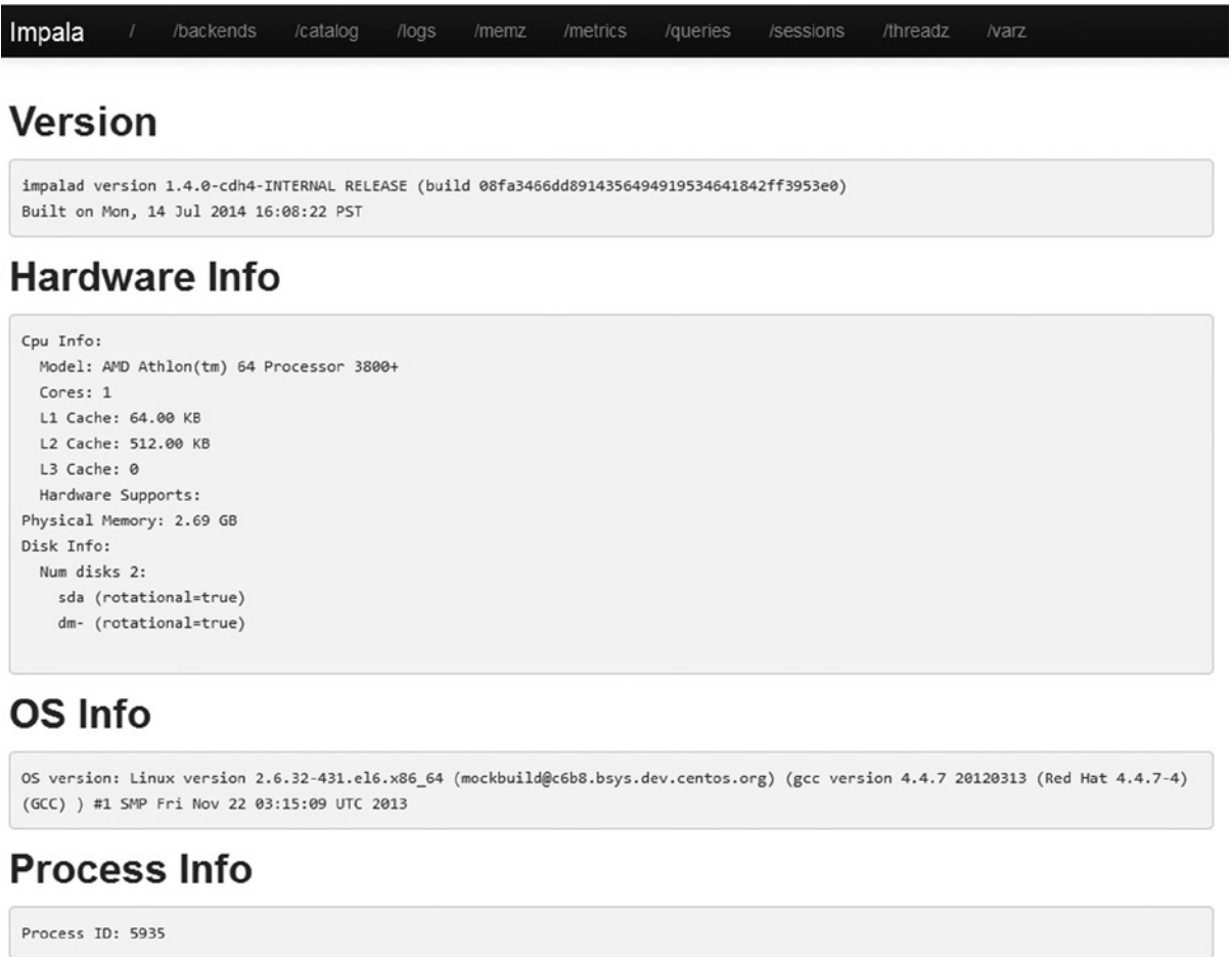
Figure 9-1. Impala server user interface
