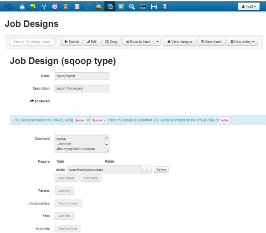
Figure 7-11. The Hue job designer: a Sqoop action
