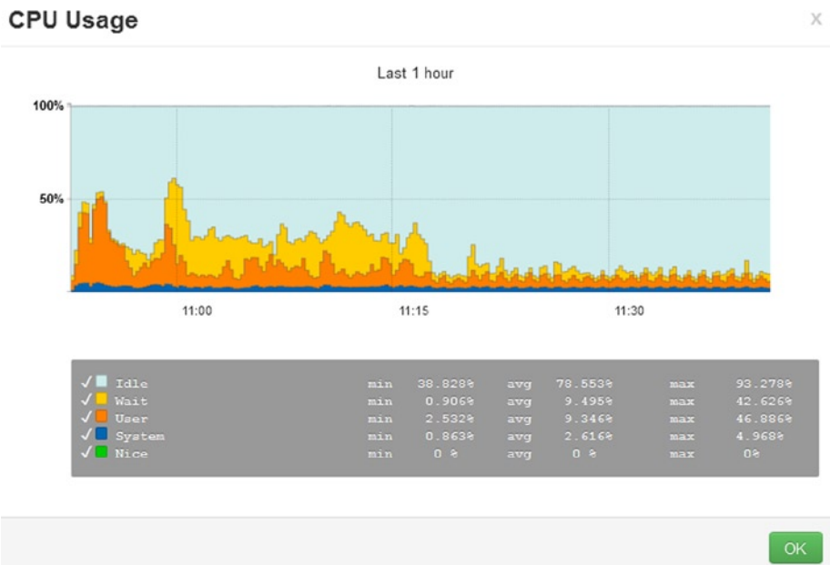
Figure 8-6. Ambari dashboard showing CPU usage
