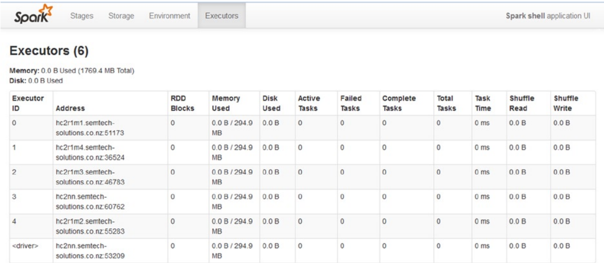
Figure 9-6. Spark application interface
