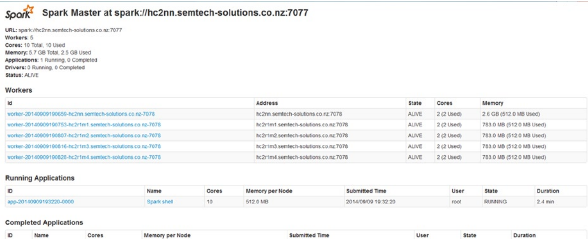
Figure 9-4. Spark Master interface with applications listed
