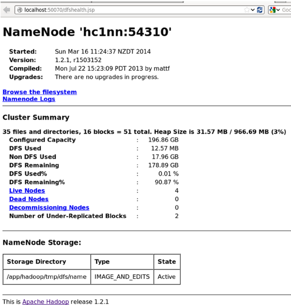
Figure 2-3. The name node user interface
