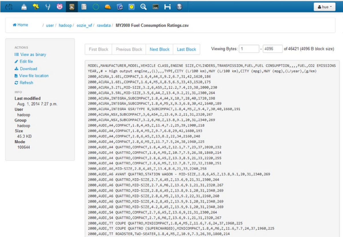
Figure 7-7. The Hue HDFS file editor
