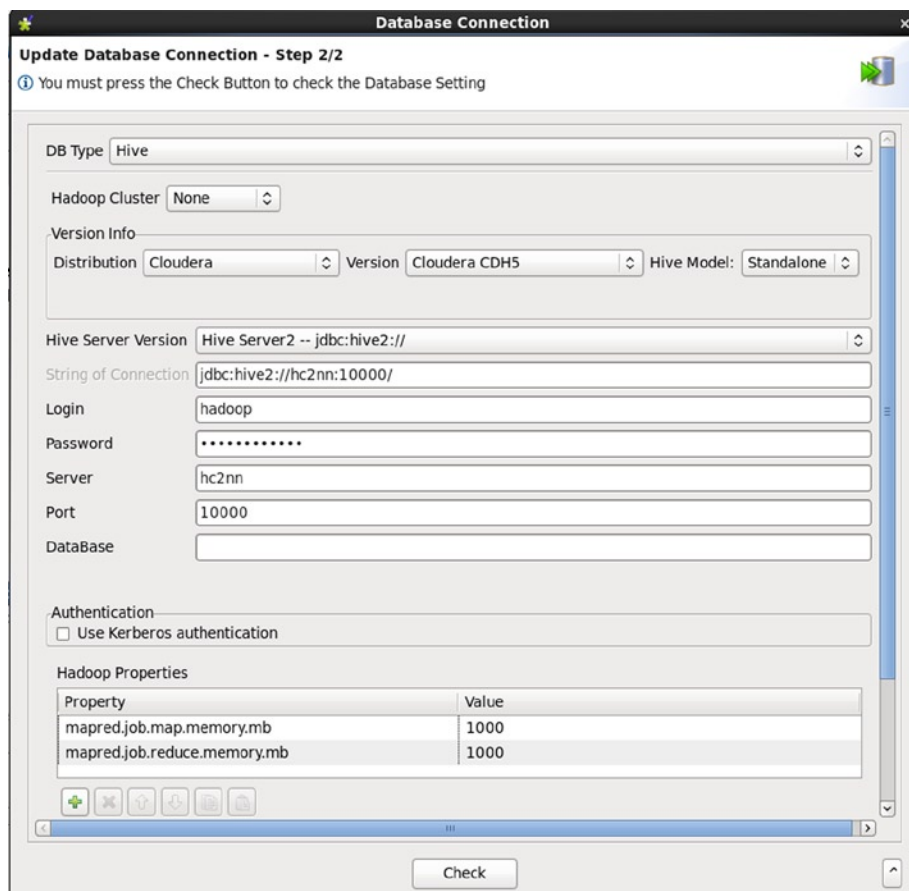
Figure 11-19. Talend-Hive database connection
