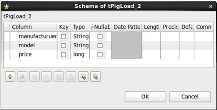
Figure 10-34. Three-column setup for trm1 job
