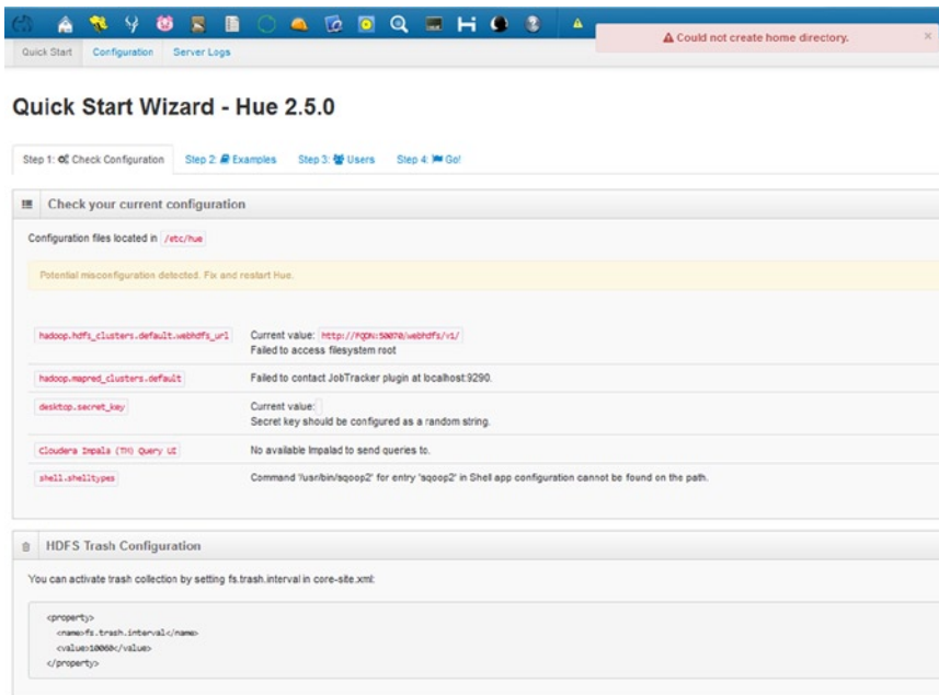
Figure 7-1. The Hue Quick Start wizard
