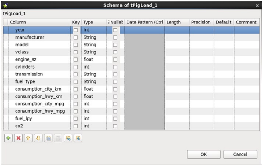
Figure 10-33. Schema window for trm1 job
