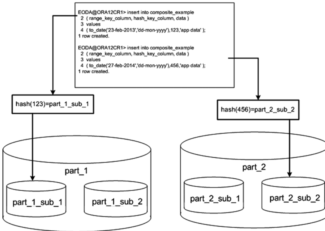
Figure 13-4. Range-hash composite partition example
