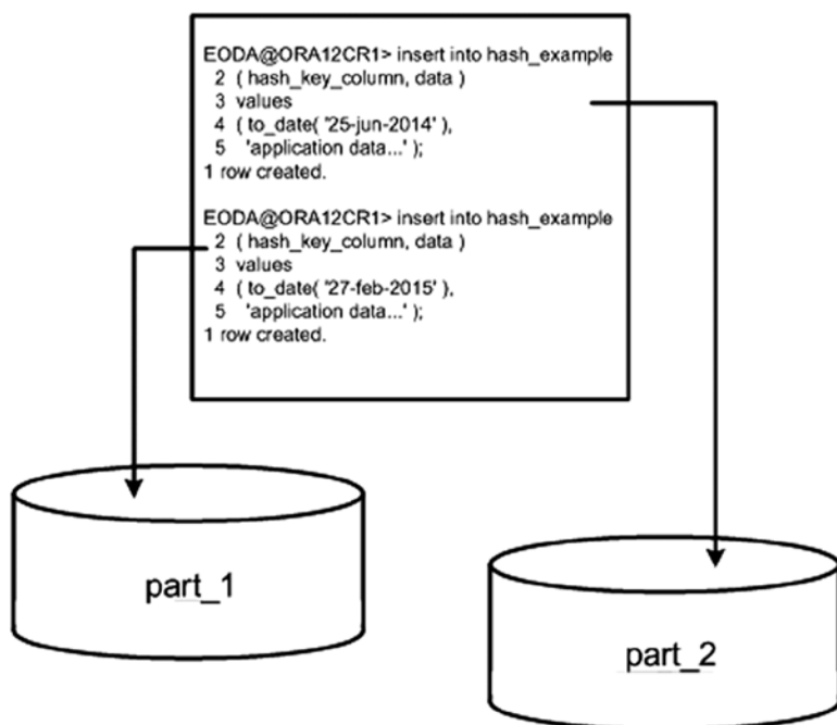
Figure 13-2. Hash partition insert example
