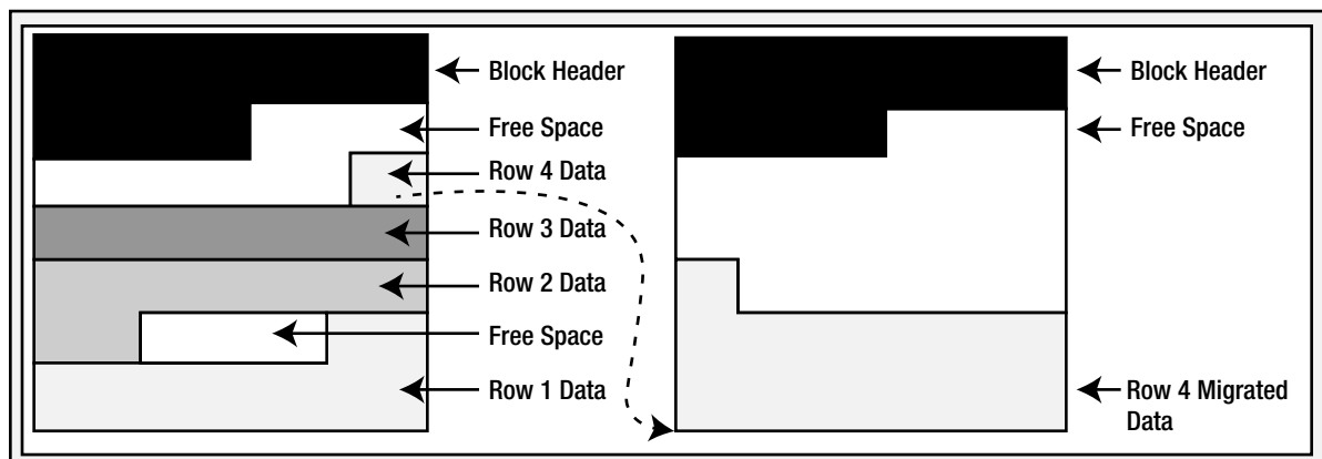
Figure 10-5. Migrated row depiction
