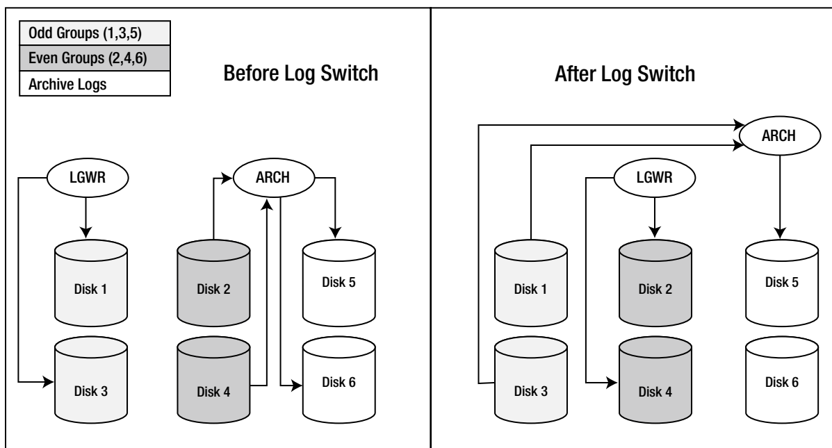
Figure 9-6. Redo log flow
