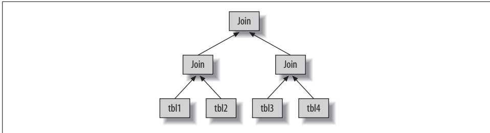
Figure 4-3. One way to join multiple tables
