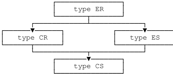
Fig. 5: Sample type graph (tuple or relation types)
