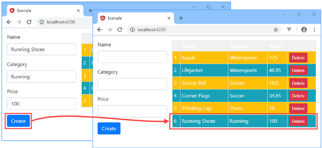
Figure 17-11. Using a custom event in a child component
