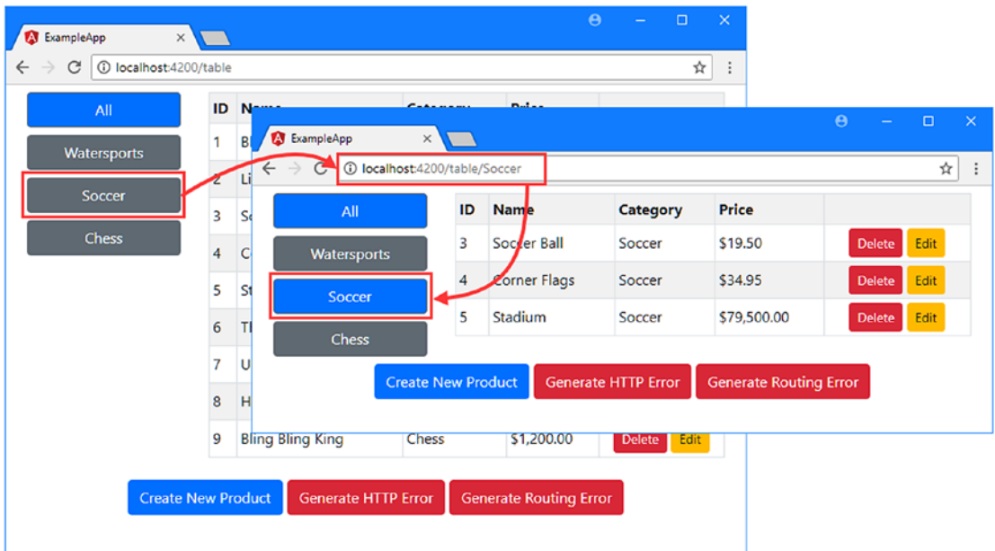
Figure 26-6. Filtering products
