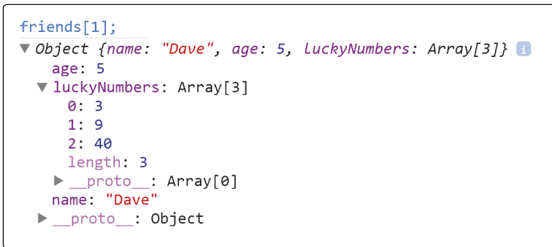
Figure 4-5: Expanding an array within the object
