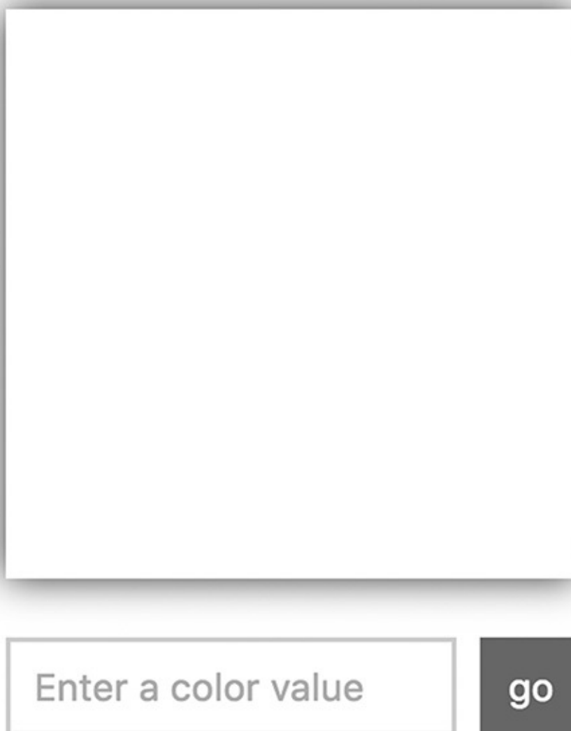
Figure 12-1 Colorizer example.
