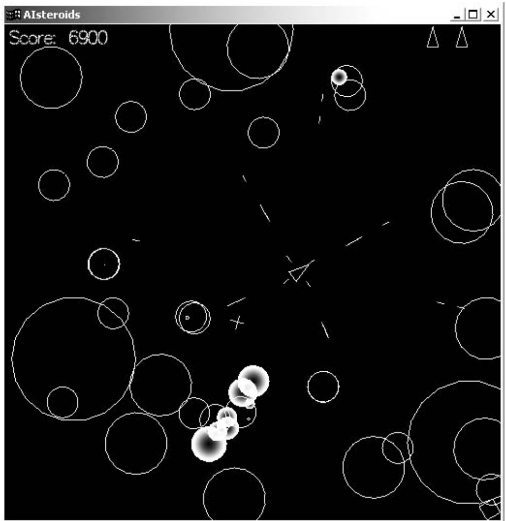
FIGURE 3.2 Asteroids screenshot.
