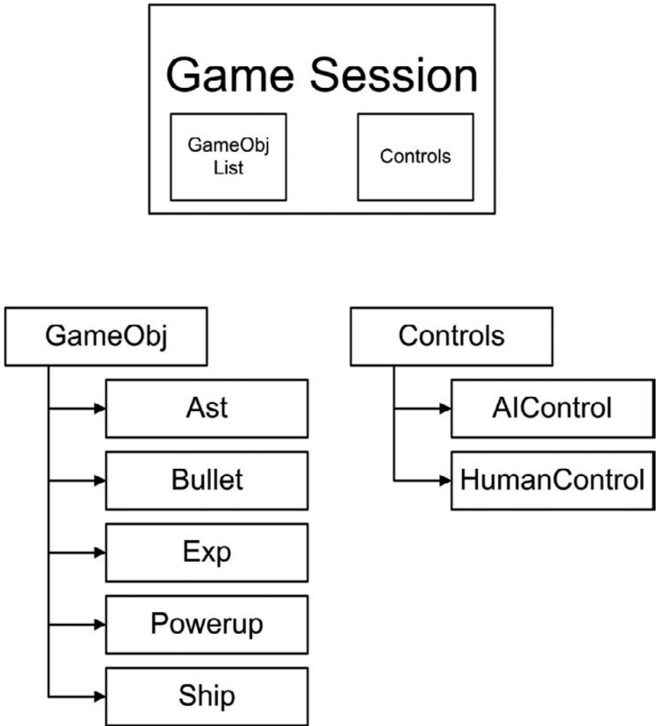
FIGURE 3.1 Asteroids class structure.
