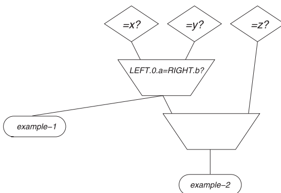
Figure 8.3 A Rete network that shares both pattern and join nodes
