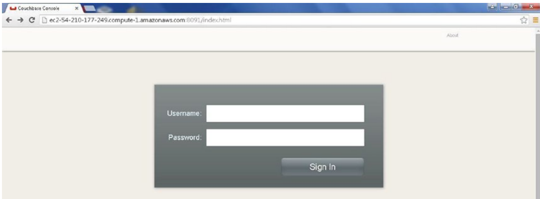
Figure 7-7. Login Page
