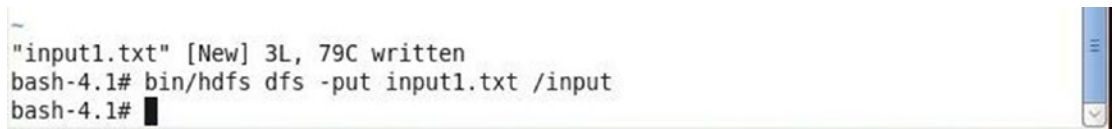
Figure 8-10. Putting the input1.txt in the HDFS
