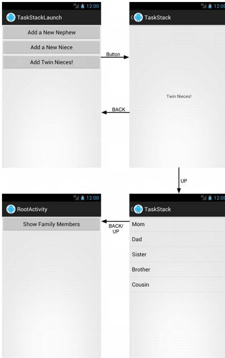
Figure 6-7. BACK versus UP navigation.
