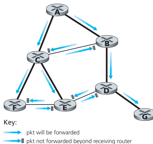
Figure 4.44 ♦ Reverse path forwarding
