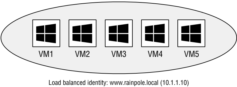
FIGURE 7.2 An NLB cluster can contain up to 32 active nodes (only 5 are shown here), and traffic is distributed equally across each available node. The NLB software allows the nodes to share a common name and IP address that is referenced by clients.
