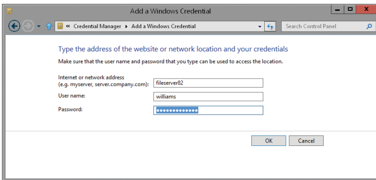
FIGURE 7-8 Create the credential entry by setting the necessary logon information.
