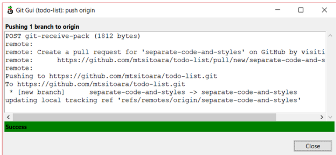
Figure 15-9. Push result
