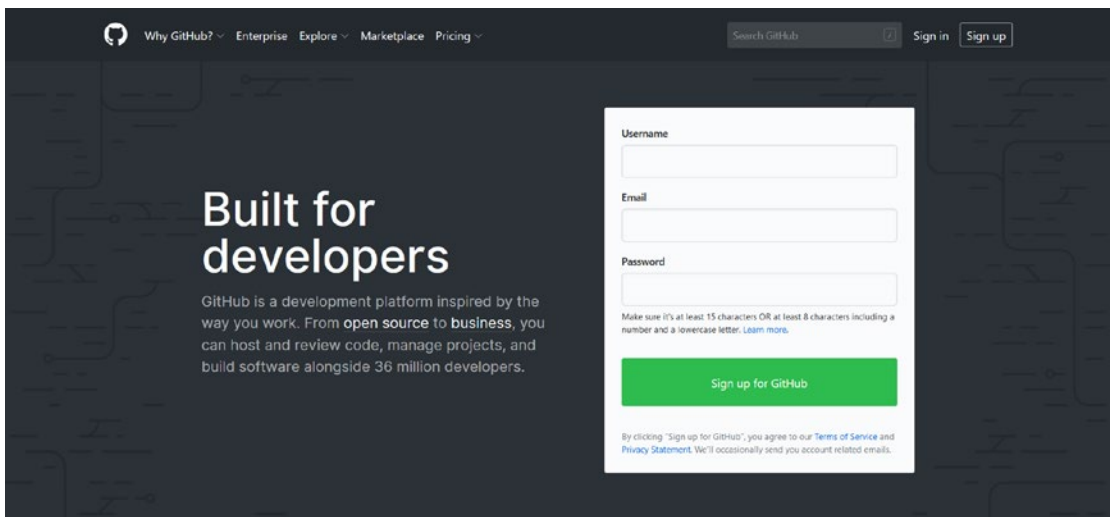
Figure 7-1. GitHub homepage
