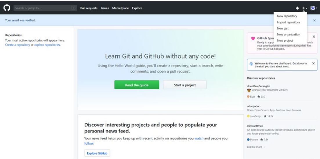
Figure 9-2. GitHub homepage
