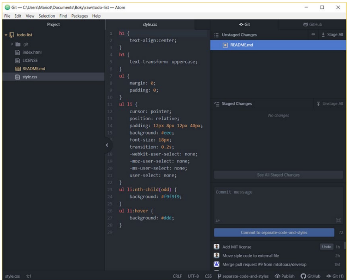
Figure 15-13. Atom interface
