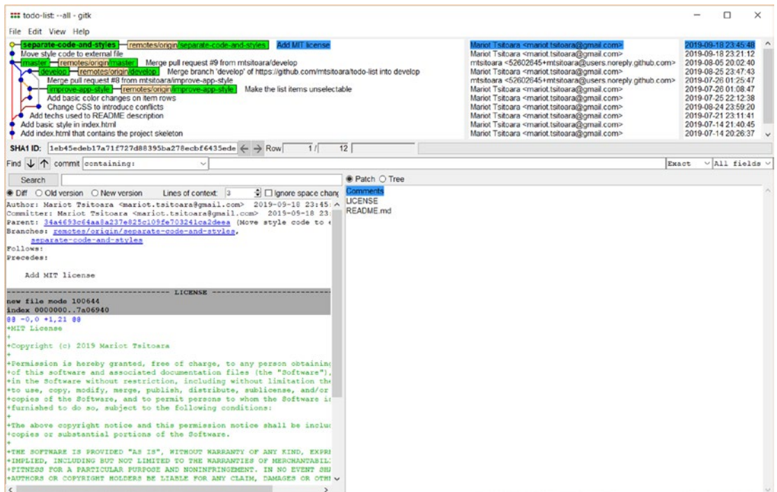
Figure 15-10. gitk interface
