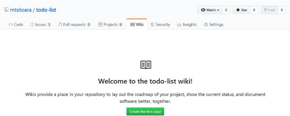
Figure 17-1. Wiki homepage
