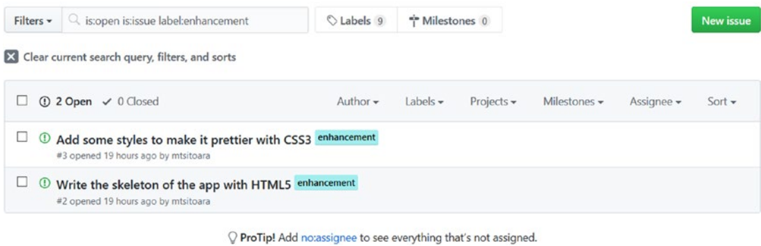
Figure 10-13. Filtered issues
