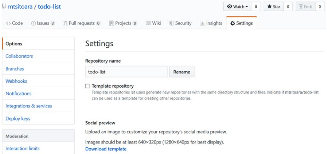
Figure 17-4. Settings page
