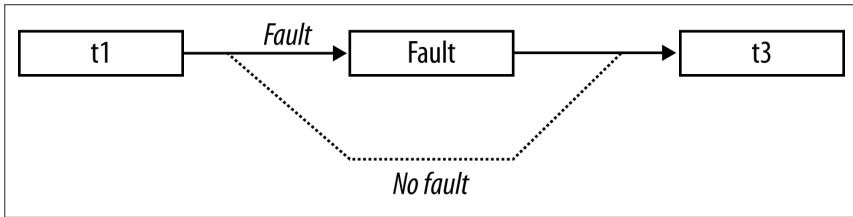
Figure 23-6. Conditional continuations
