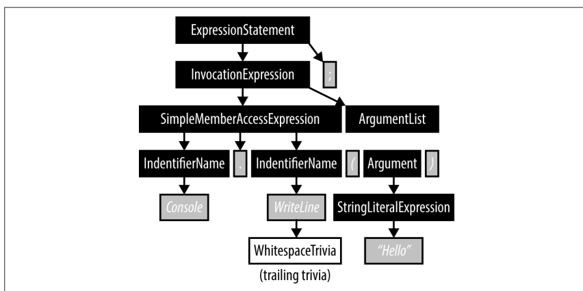
Figure 27-1. Syntax trees
