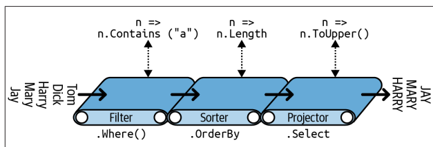
Figure 6. Chaining query operators
