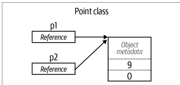
Figure 4. Assignment copies a reference
