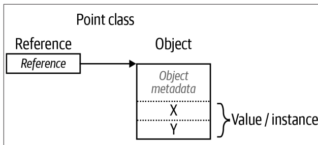
Figure 3. A reference type instance in memory
