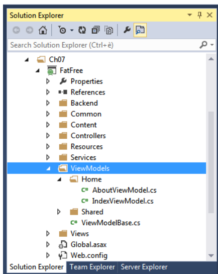
FIGURE 2-6 A suggested structure for the ViewModels folder.
