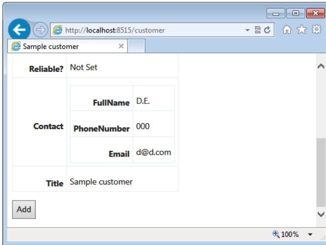
FIGURE 4-10 Nested models.
