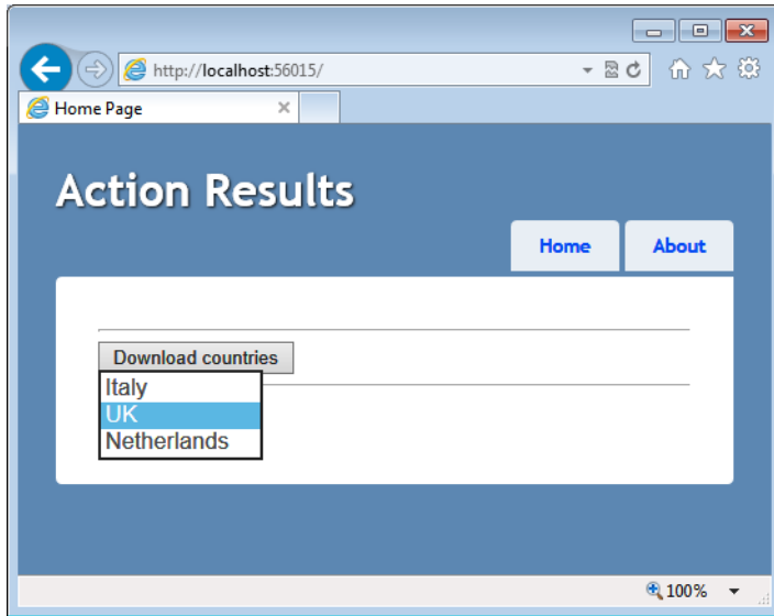
FIGURE 8-7 A drop-down list populated with Ajax-retrieved JSON data.
