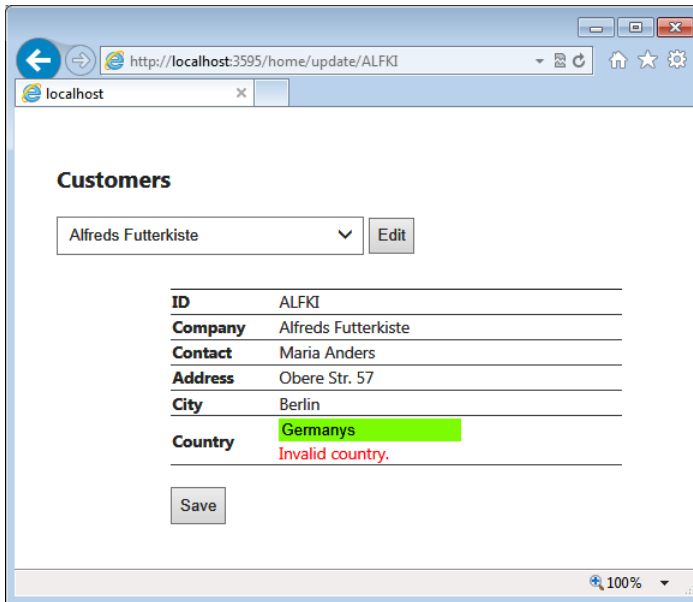
FIGURE 4-3 Handling invalid input.
