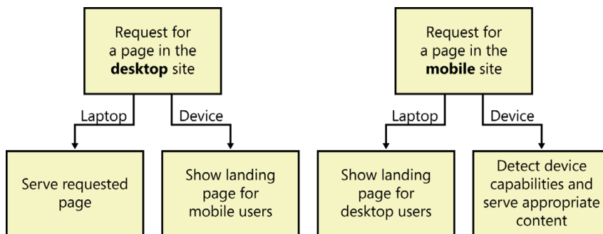
FIGURE 12-13 The desktop/mobile view switcher algorithm.
