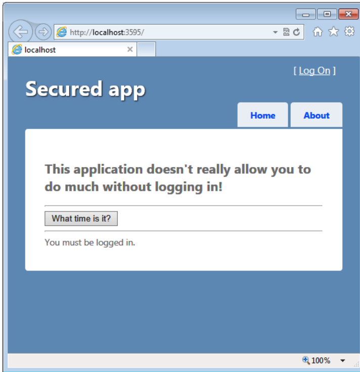
FIGURE 6-3 No logon view shows up in case of Ajax requests.
