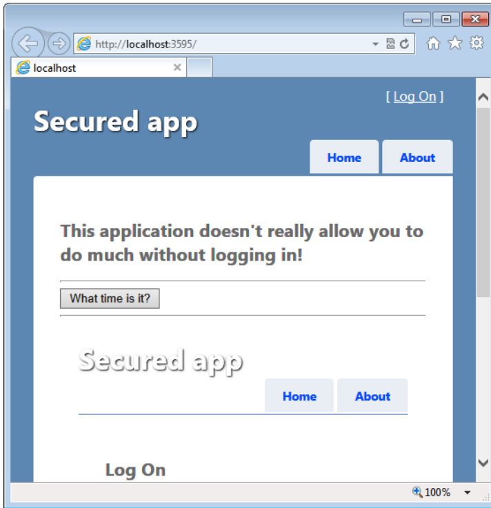
FIGURE 6-2 An Ajax request to a restricted URL injects the logon view.
