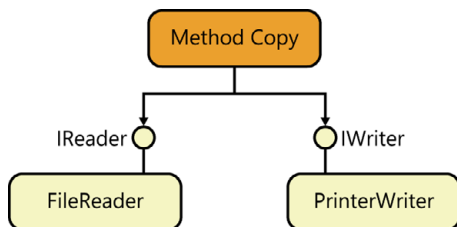
FIGURE 7-6 The DIP diagram.
