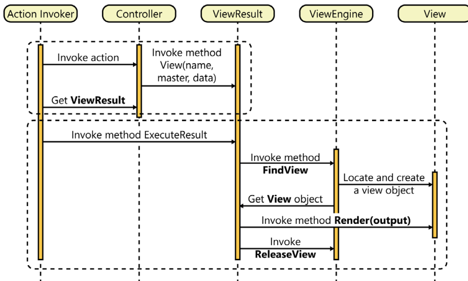
FIGURE 2-3 A sequence diagram that illustrates the request-servicing process.
