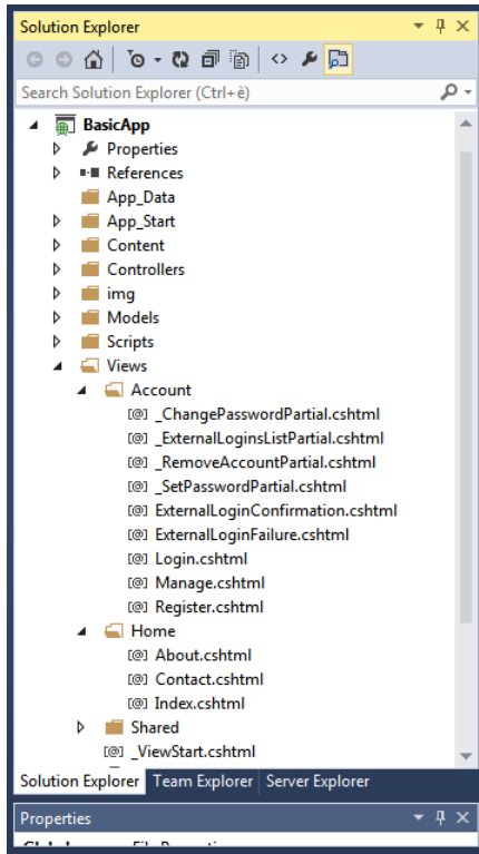
FIGURE 2-4 Locating view templates in an ASP.NET MVC application.
