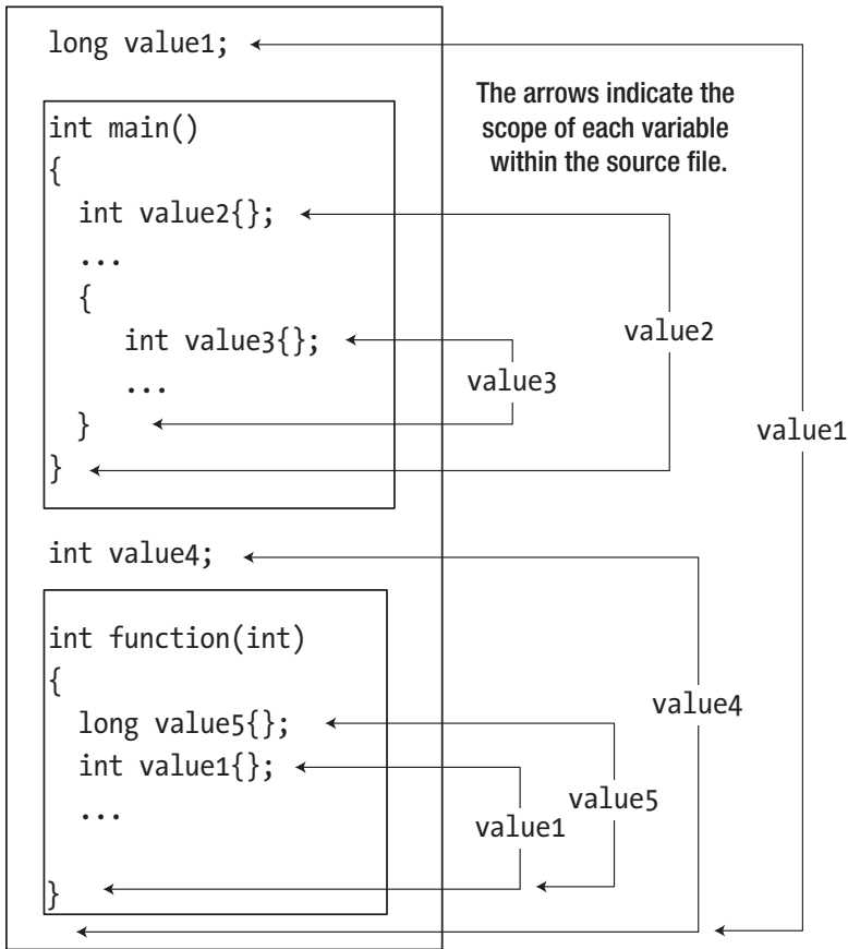
Figure 3-3. Variable scope
