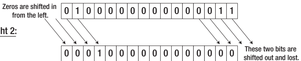
Figure 3-2. Shift operations
