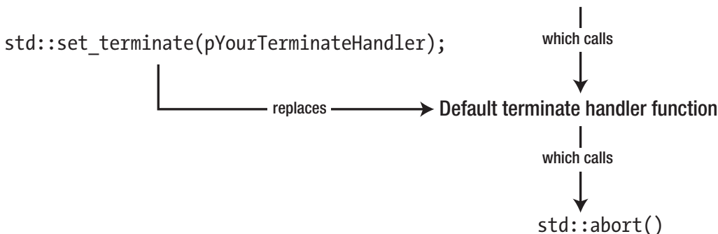
Figure 16-7. Uncaught exceptions
