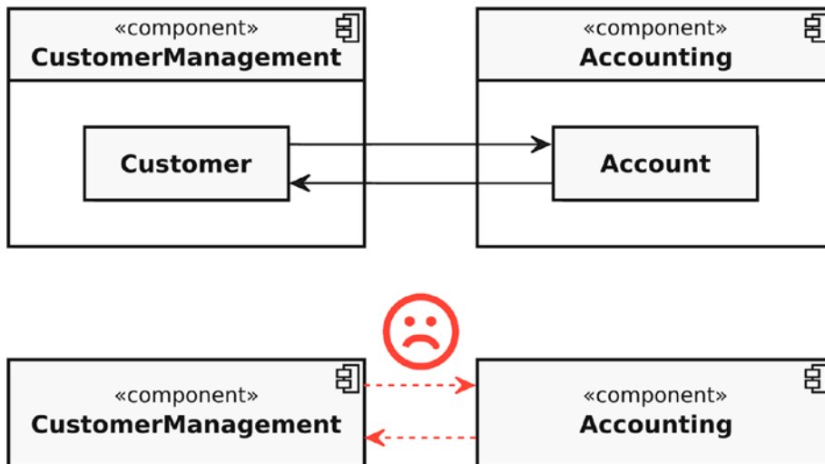
Figure 6-5. The impact of circular dependencies between classes in different components
