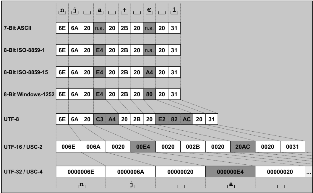
Figure 16.1. Hexadecimal Character Codes of Different Character Sets
