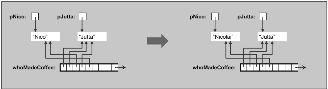
Figure 5.1. Using shared_ptr s
