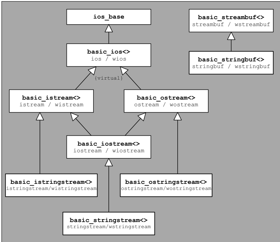
Figure 15.3. Class Hierarchy of the String Stream Classes
