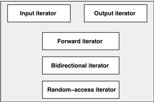
Figure 9.1. Iterator Categories
