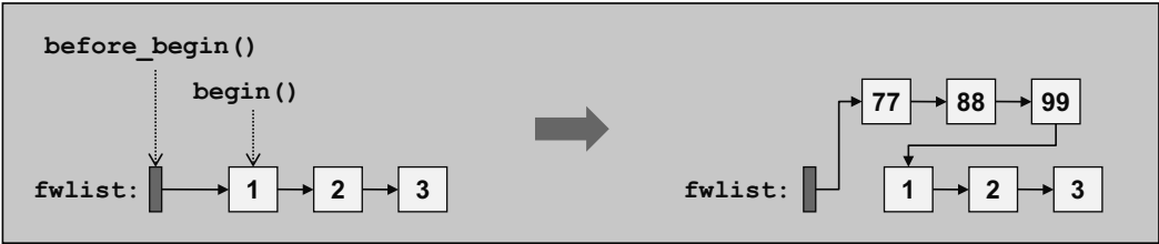
Figure 7.9. Inserting Elements at the Beginning of a Forward List
