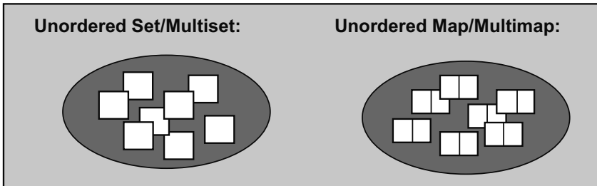
Figure 7.16. Unordered Containers
