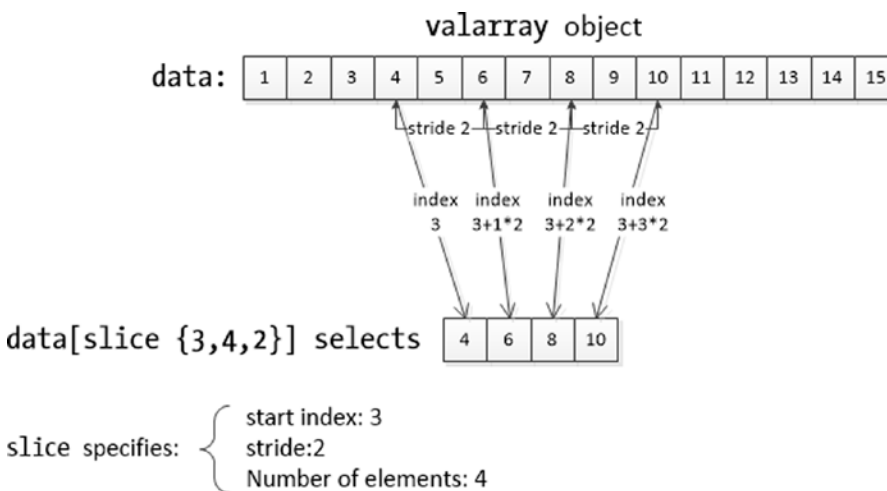
Figure 10-3. Subset of elements in a valarray selected by a slice object
