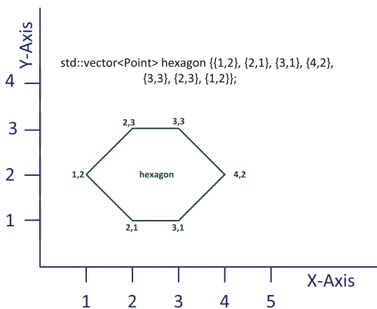
Figure 7-4. A polyline that represents a hexagon
