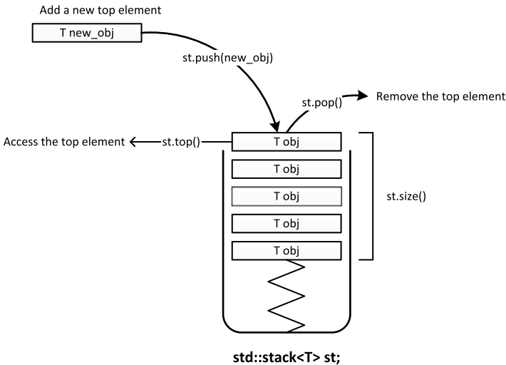
Figure 3-1. Basic stack container operations
