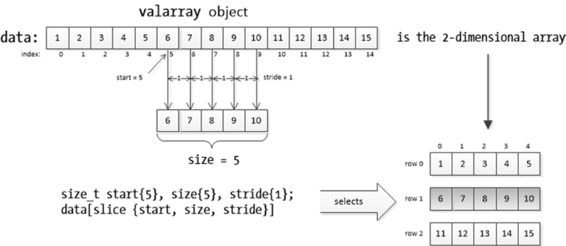
Figure 10-4. Selecting a single row of a two-dimensional array
