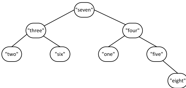
Figure 5-2. Balanced binary tree of strings ordered by greater<string>
