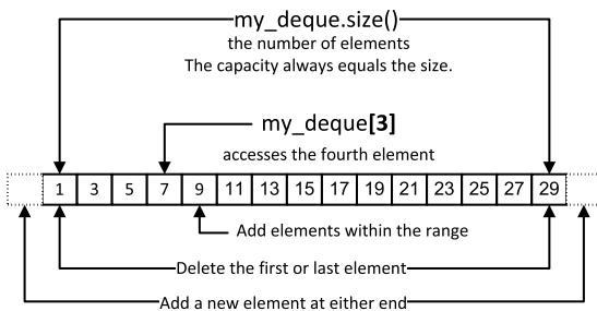
Figure 2-5. An example of a deque container
