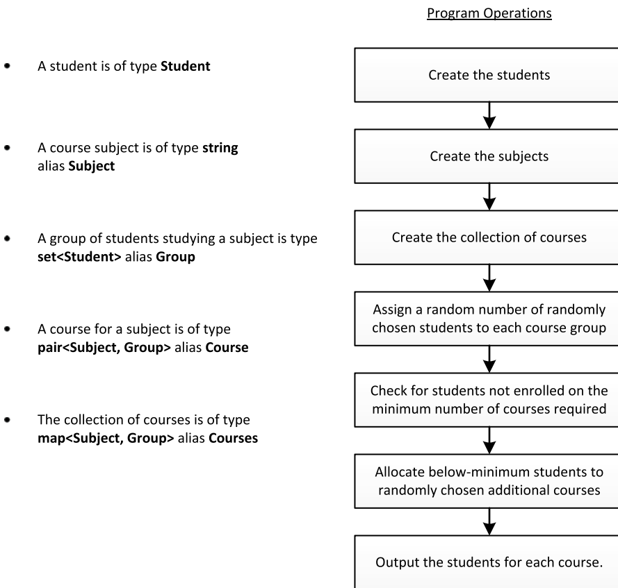
Figure 5-3. Operations in the example using set containers to represent course groups
