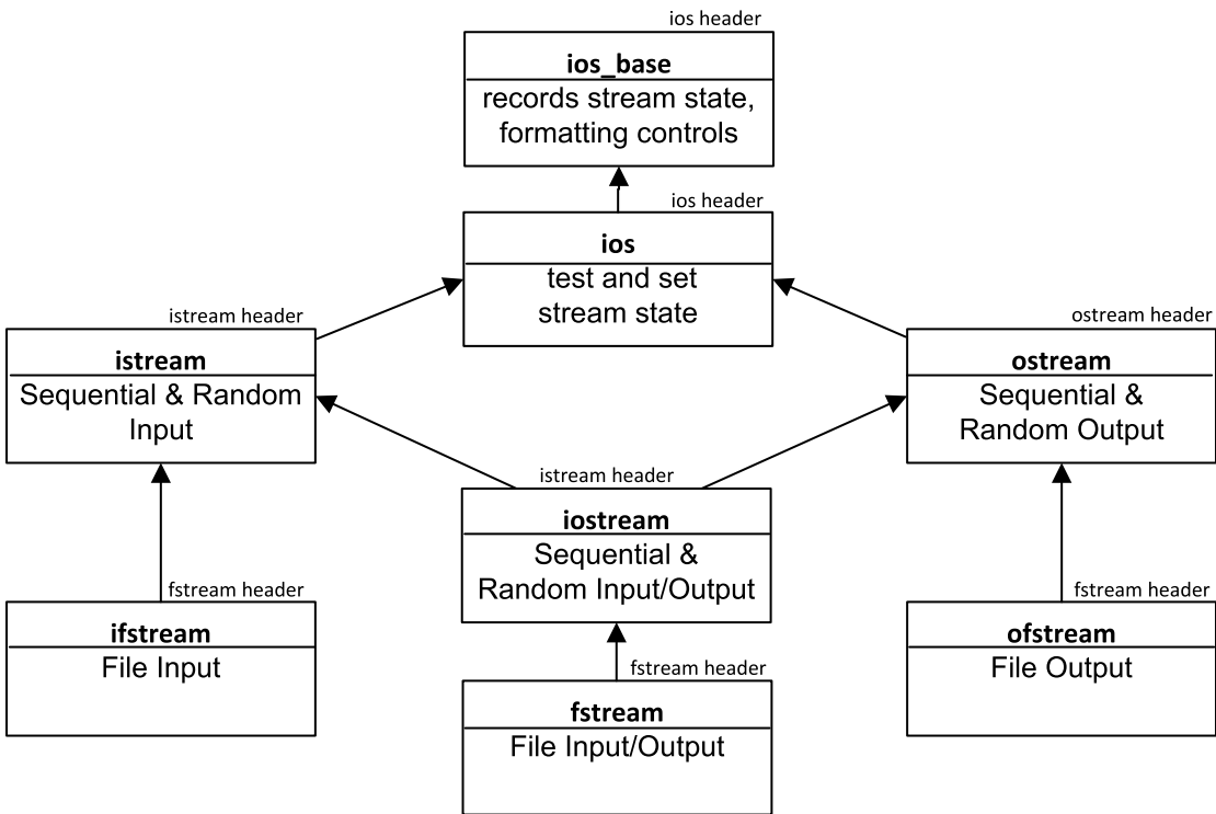
Figure 9-1. Inheritance hierarchy for class templates that represent file streams
