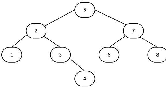
Figure 5-1. Balanced binary tree of integers ordered by less<int>
