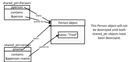
Figure 5-4. A shared pointer that points to a different object from the object it owns
