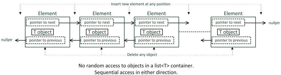
Figure 2-6. Organization of elements in a list<T> container
