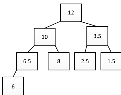
Figure 3-5. The tree that a heap represents
