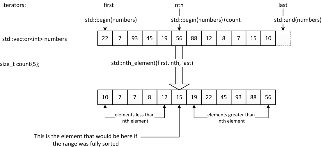
Figure 6-2. Operation of the nth_element() algorithm
