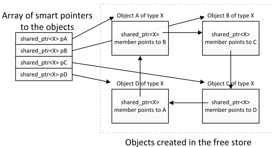
Figure 1-4. How a reference cycle prevents objects from being deleted
