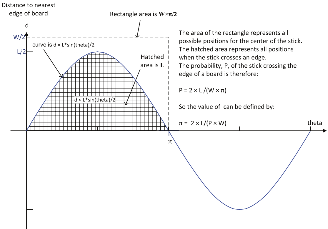
Figure 8-4. Determining \pi from the probability of the stick crossing an edge of a floorboard
