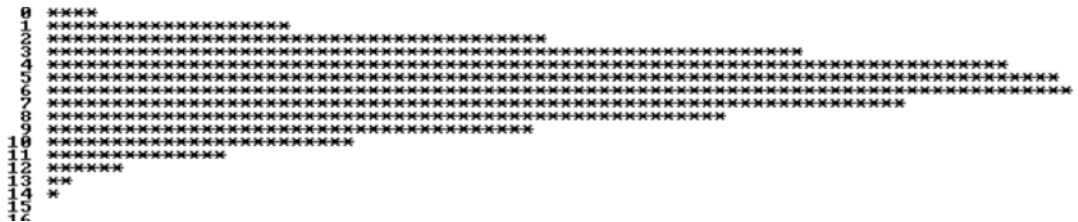
Weibull Distribution - a = 2.5 b = 7.0
