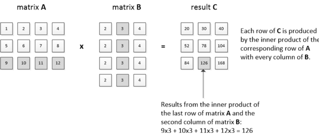
Figure 10-1. Matrix multiplication and the inner product operation
