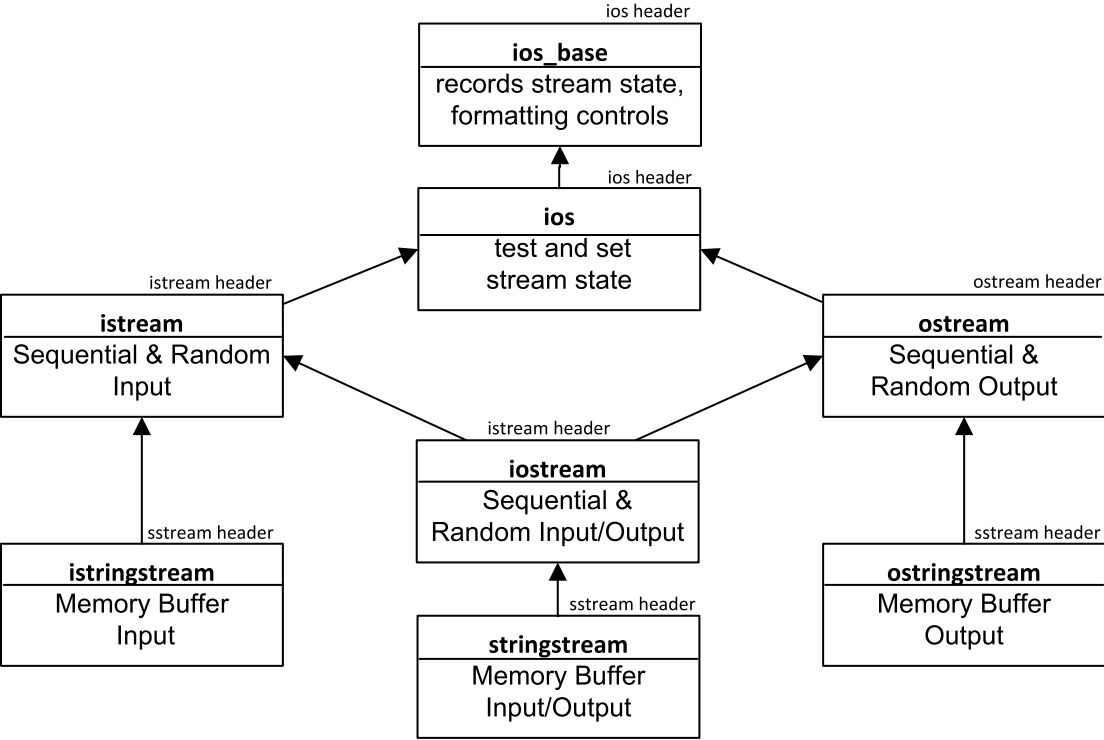
Figure 9-2. Inheritance hierarchy for string stream types
