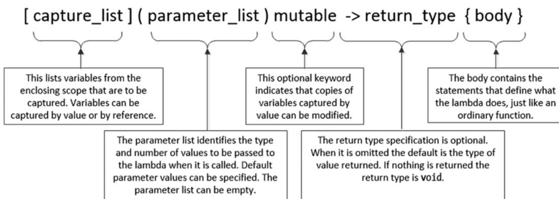
Figure 1-5. Components of a lambda expression
