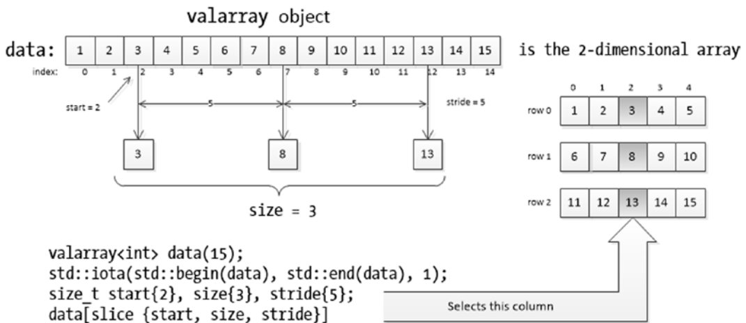
Figure 10-5. Selecting a single column from a two-dimensional array
