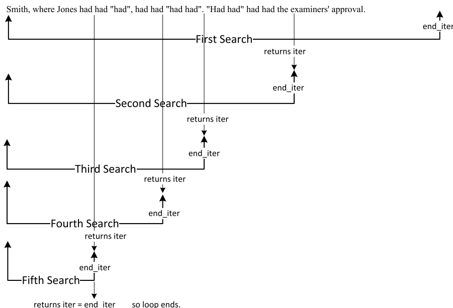
Figure 6-5. Searching repeatedly with find_end()
