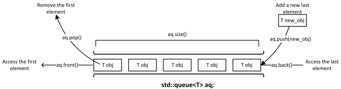
Figure 3-2. A queue container
