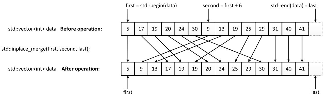
Figure 6-4. inplace_merge() operation
