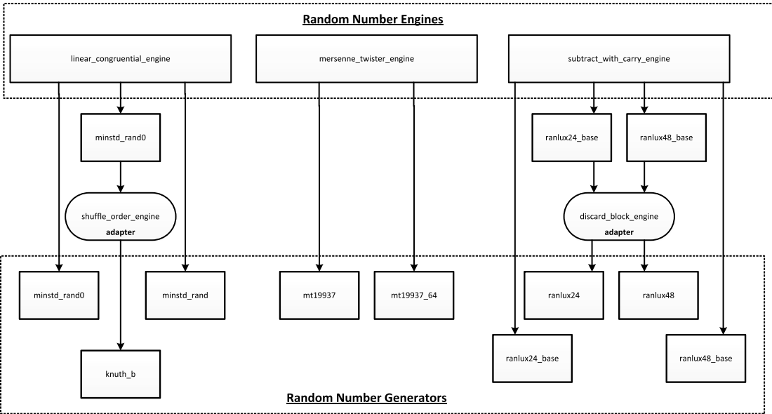
Figure 8-12. The connection between random number generators and random number engines
