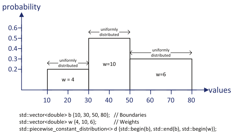
Figure 8-7. The piecewise constant distribution
