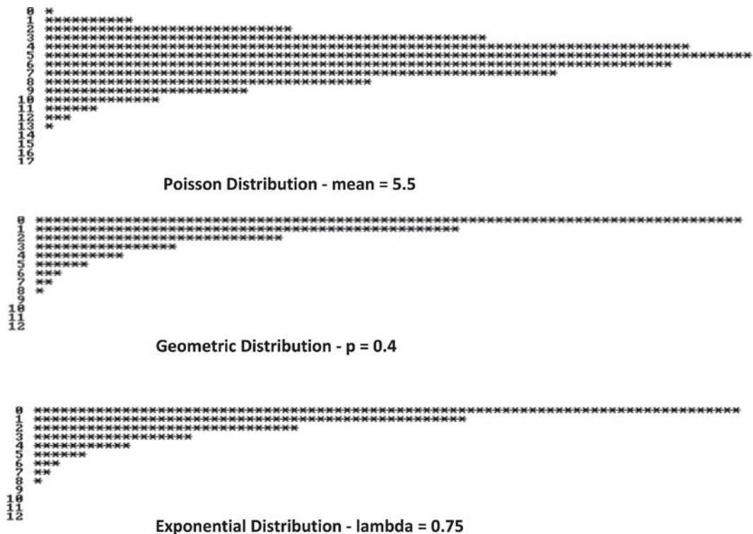
Figure 8-9. Examples of Poisson, geometric, and exponential distributions
