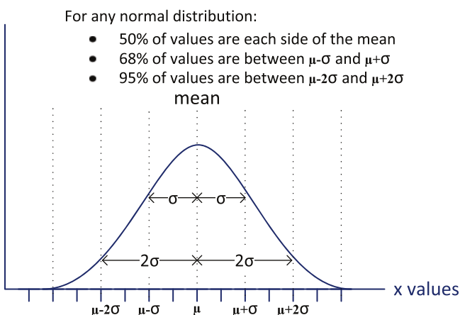
Figure 8-5. The normal distribution
