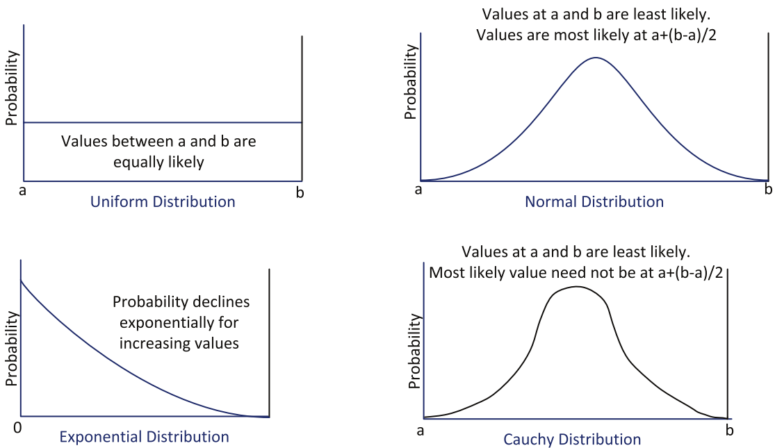
Figure 8-1. Examples of distributions
