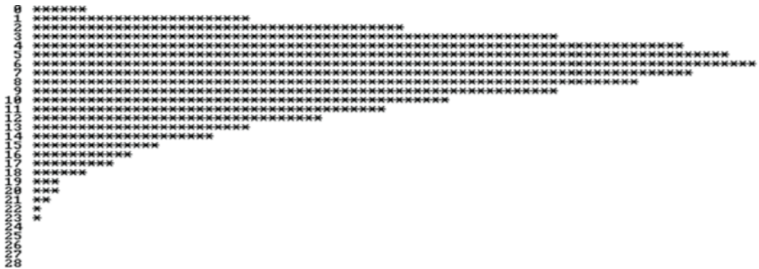
Negative Binomial Distribution - k = 5 p = 0.4
