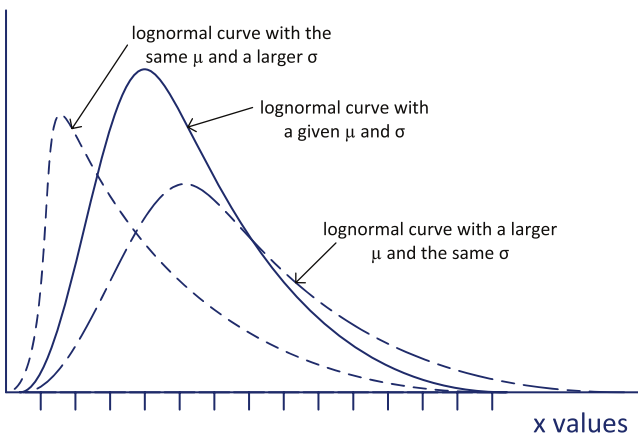
Figure 8-6. Lognormal distributions
