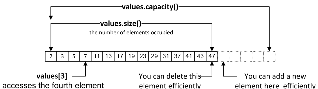
Figure 2-3. The size and capacity of a vector
