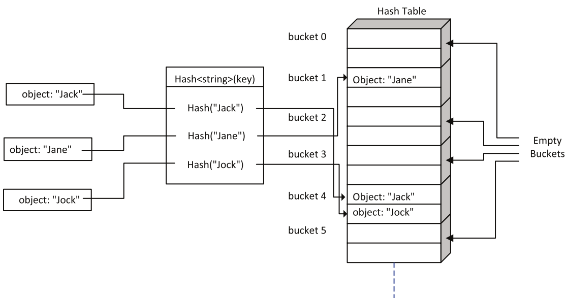
Figure 5-5. Conceptual data organization in an unordered_set container
