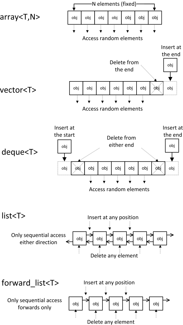
Figure 2-1. The standard sequence containers
