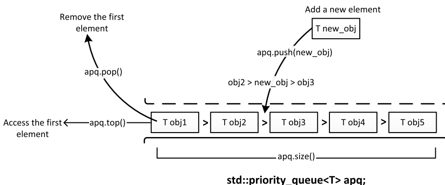
Figure 3-3. A priority_queue container
