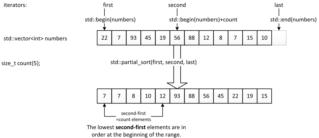
Figure 6-1. Operation of the partial_sort() algorithm
