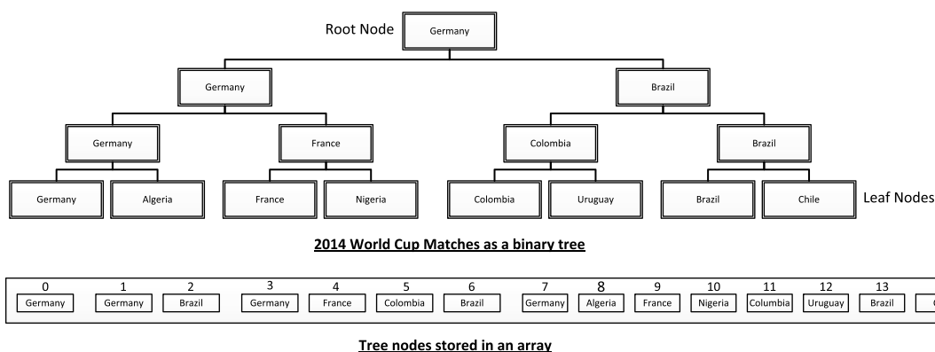
Figure 3-4. Example of a binary tree
