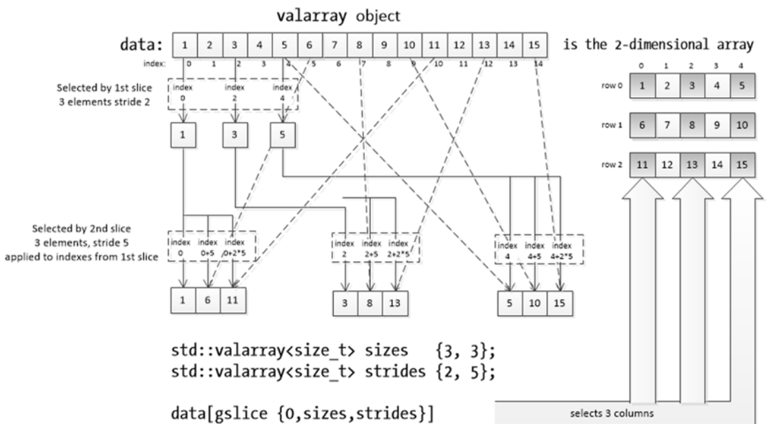
Figure 10-12. Selecting multiple columns from a two-dimensional array
