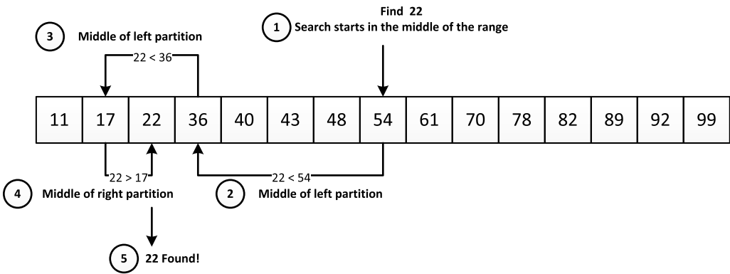
Figure 6-6. A binary search
