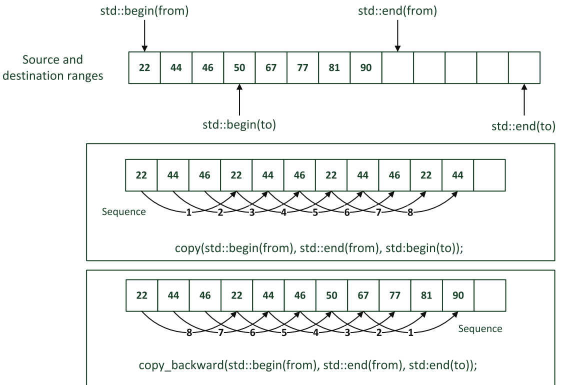
Figure 7-2. Copying overlapping ranges to the right
