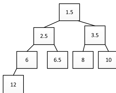
The tree that the sorted heap represents
