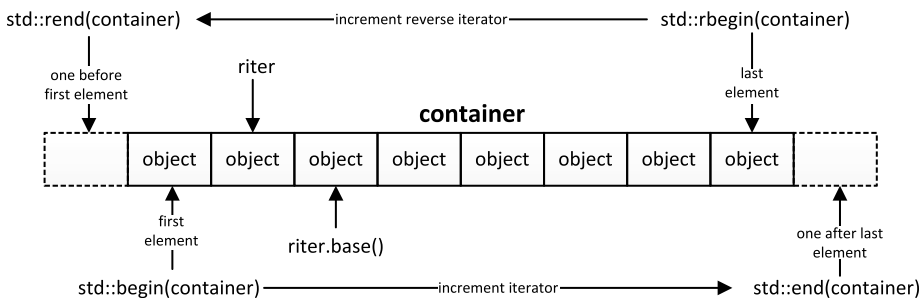
Figure 1-3. How iterators and reverse iterators relate to a container
