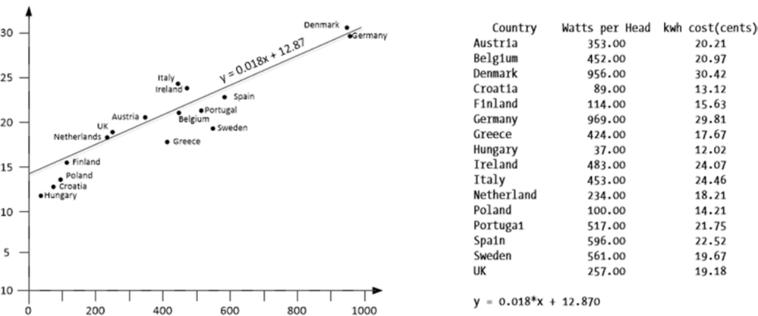
Figure 10-2. Result of least squares linear regression
