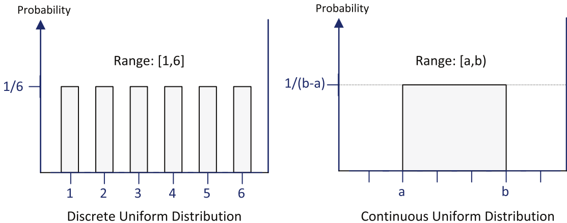
Figure 8-2. Uniform distributions
