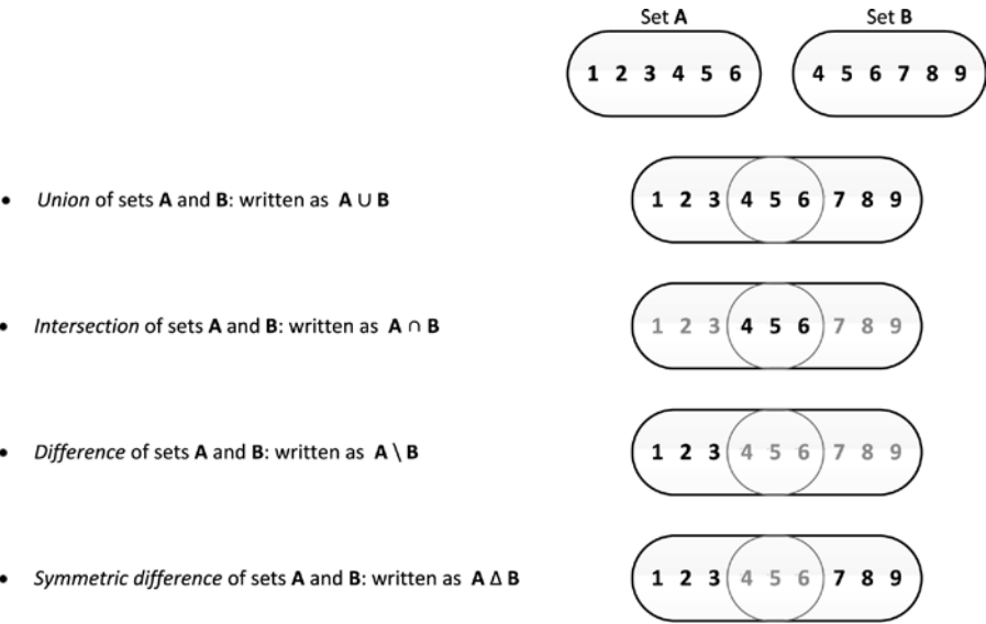
Figure 5-6. Set operations
