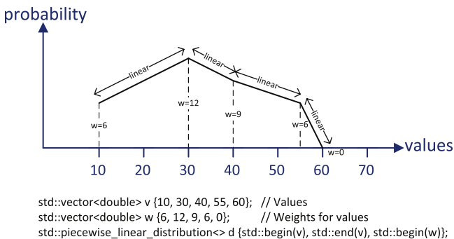
Figure 8-8. A piecewise linear distribution
