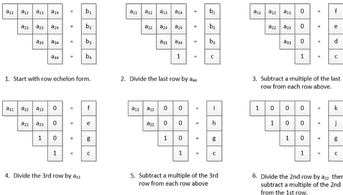
Figure 10-10. Back substitution
