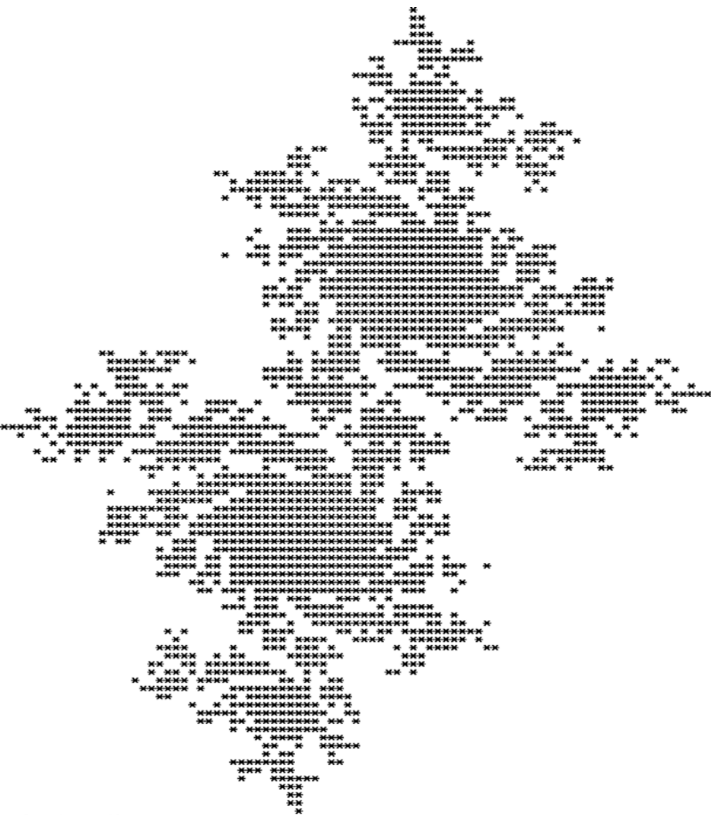
Figure 10-13. The Julia set generated by Ex10-06
