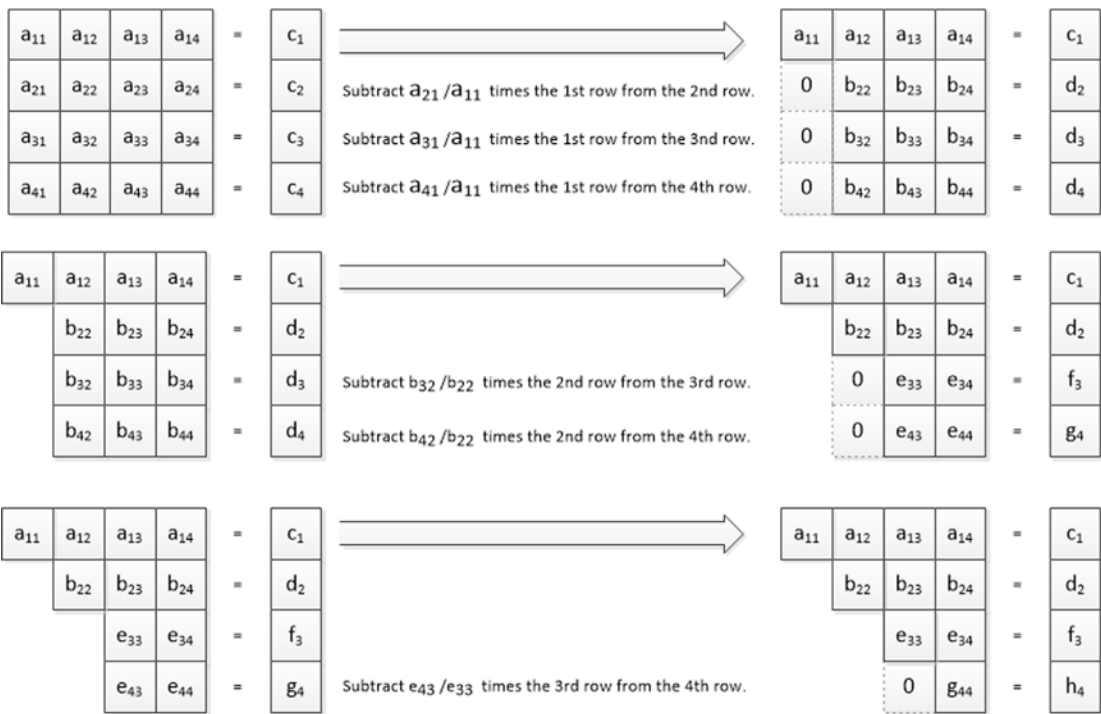
Figure 10-7. Transforming linear equations into row echelon form
