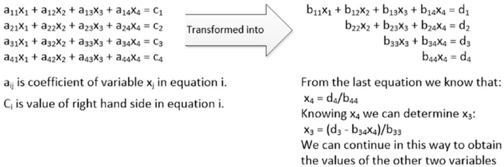
Figure 10-6. What the Gaussian Elimination method does
