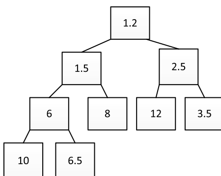
Figure 3-6. A heap of floating-point values
