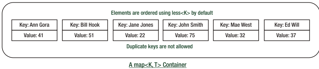
Figure 4-1. A conceptual representation of a map<K,T> container
