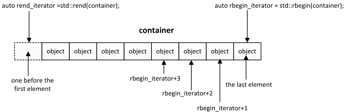
Figure 1-2. Operations with reverse iterators
