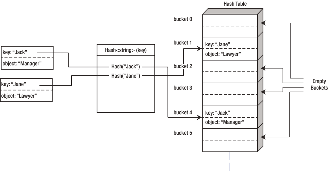
Figure 4-3. Data in an unordered_map
