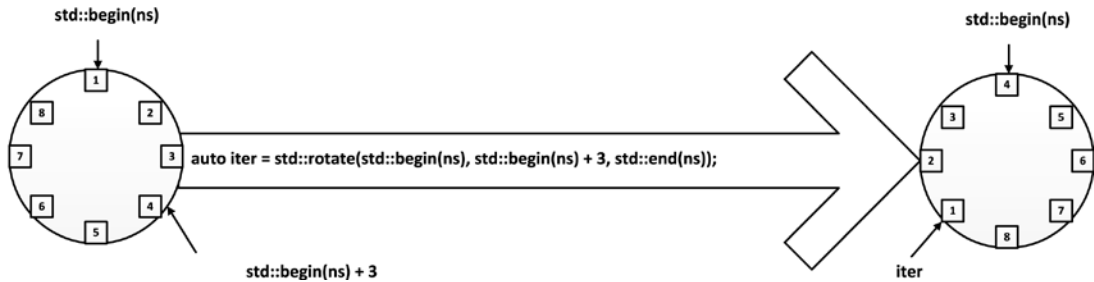
Figure 7-3. How the rotate() algorithm works
