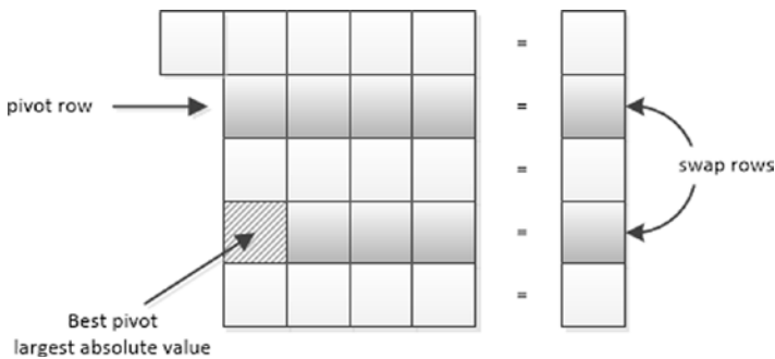
Figure 10-8. Choosing the best pivot
