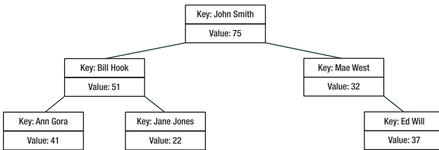
Balanced Binary Tree for a map Container
