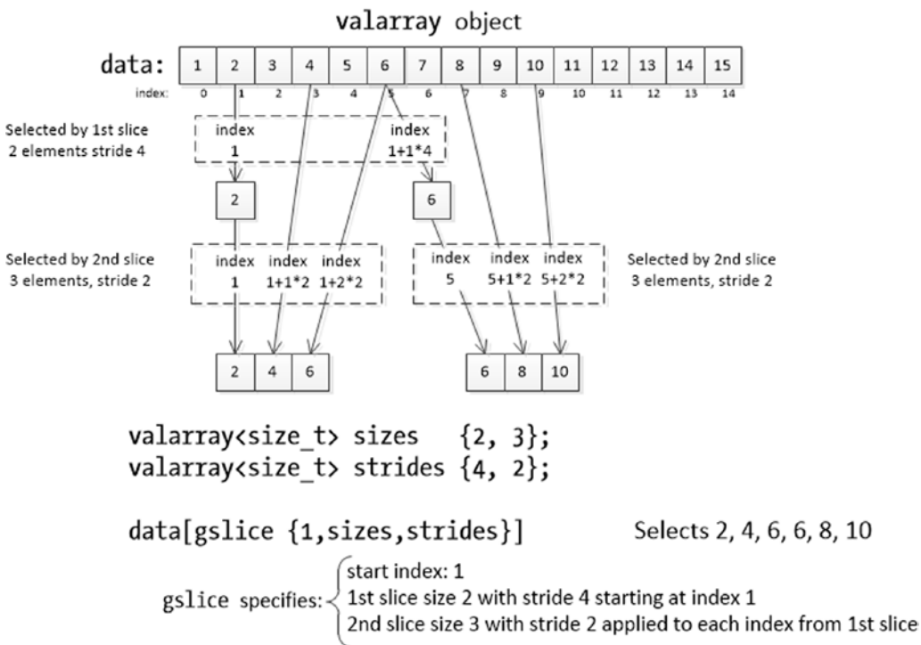
Figure 10-11. How a gslice object selects elements from a valarray
