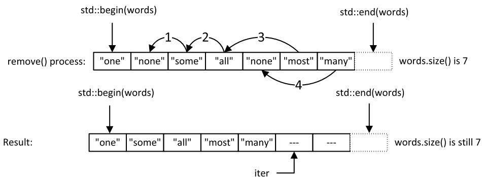
Figure 2-4. How the remove() algorithm works
