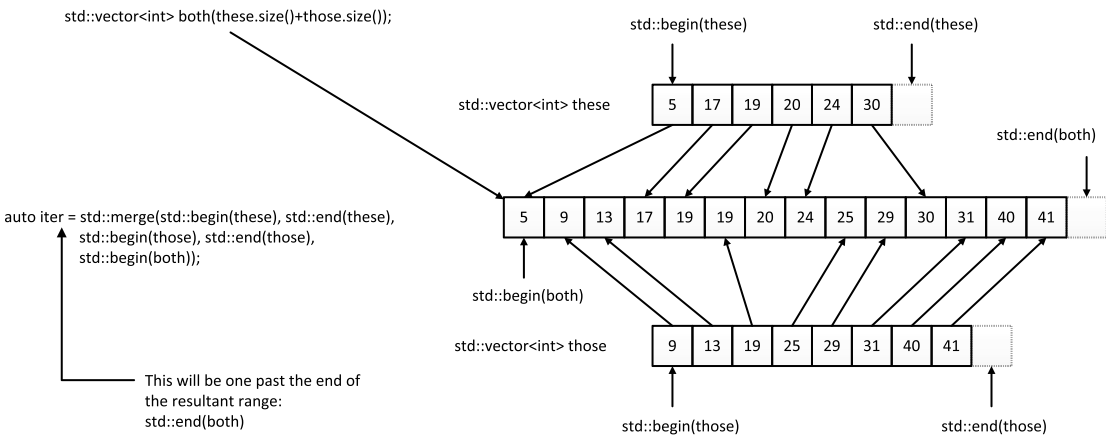
Figure 6-3. Merging elements from two vector containers
