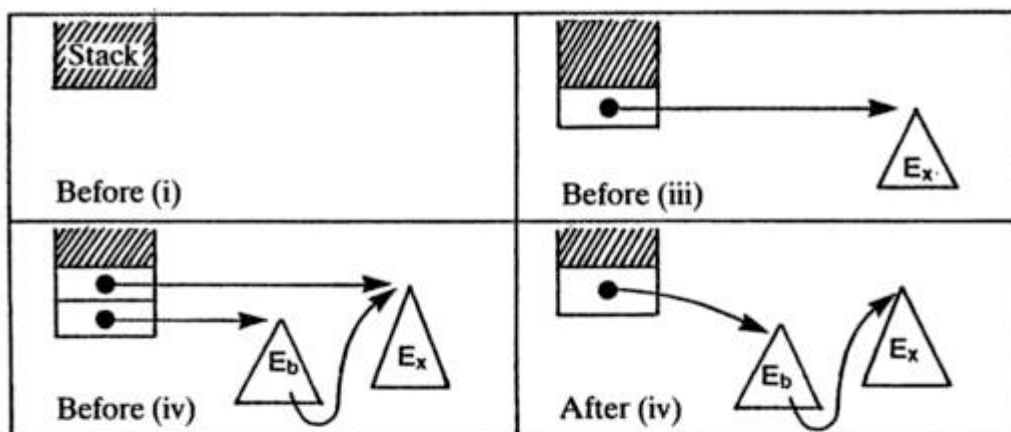
Figure 18.8 Execution of a let
