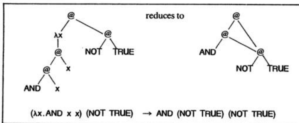
Figure 12.2 Pointer substitution
