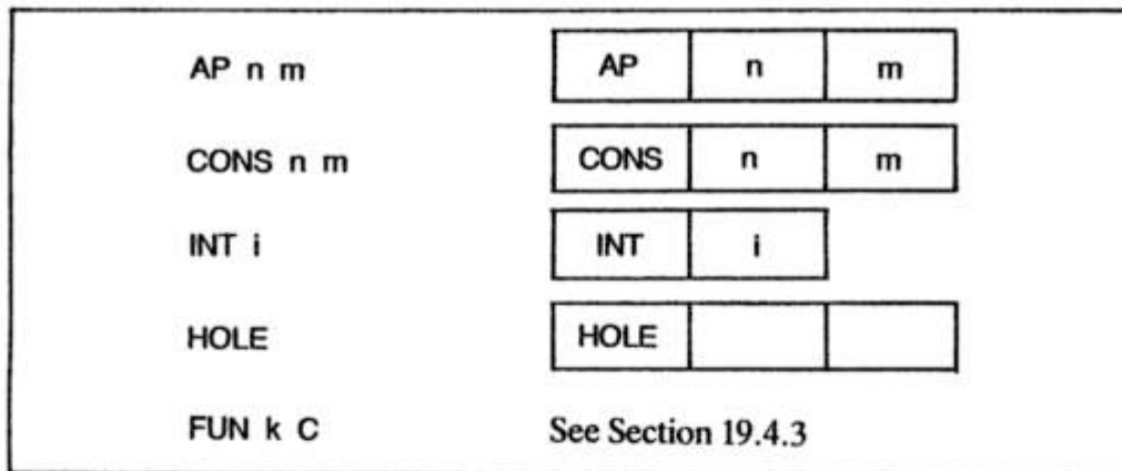
Figure 19.3 Node representations in the G-machine
