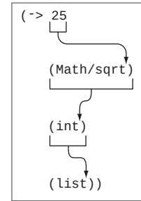
Figure 8.1 Arrow macro: each expression is inserted into the following one at compile time, allowing you to write the whole expression inside-out when that feels more natural.
