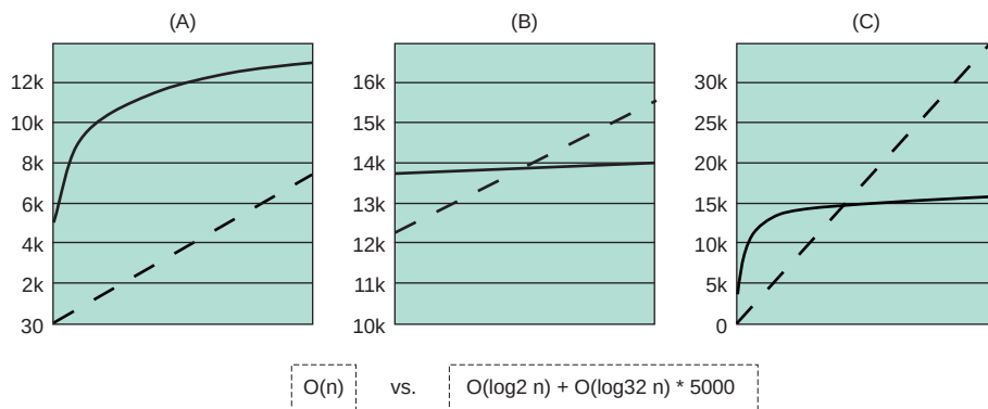
Figure 5.2 In Big-O, regardless of the other ancillary costs, the higher order of magnitude always overtakes the lower eventually.
