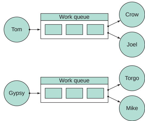
Figure 11.2 The concurrent design can be parallelized through the use of another work queue and producer as well as two more consumers.
