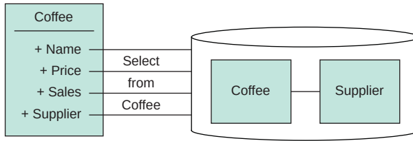
Figure 14.2 Via various programming magicks, an ORM provides a class-instance interface that maps to database tables on the back end for its property values.
