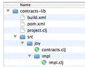
Figure 9.4 Private API directories: using the folder layout to hide namespace implementation details
