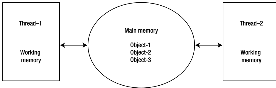
Figure 6-5. Java Memory model
