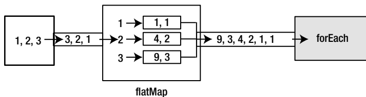
Figure 13-8. Flattening a stream using the flatMap() method
