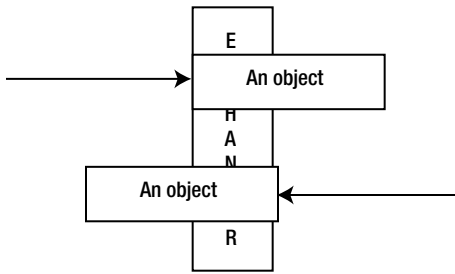
Figure 6-15. Two threads meet at exchange point and exchange objects
