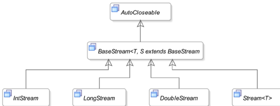
Figure 13-6. A class diagram for stream-related interfaces in the Streams API
