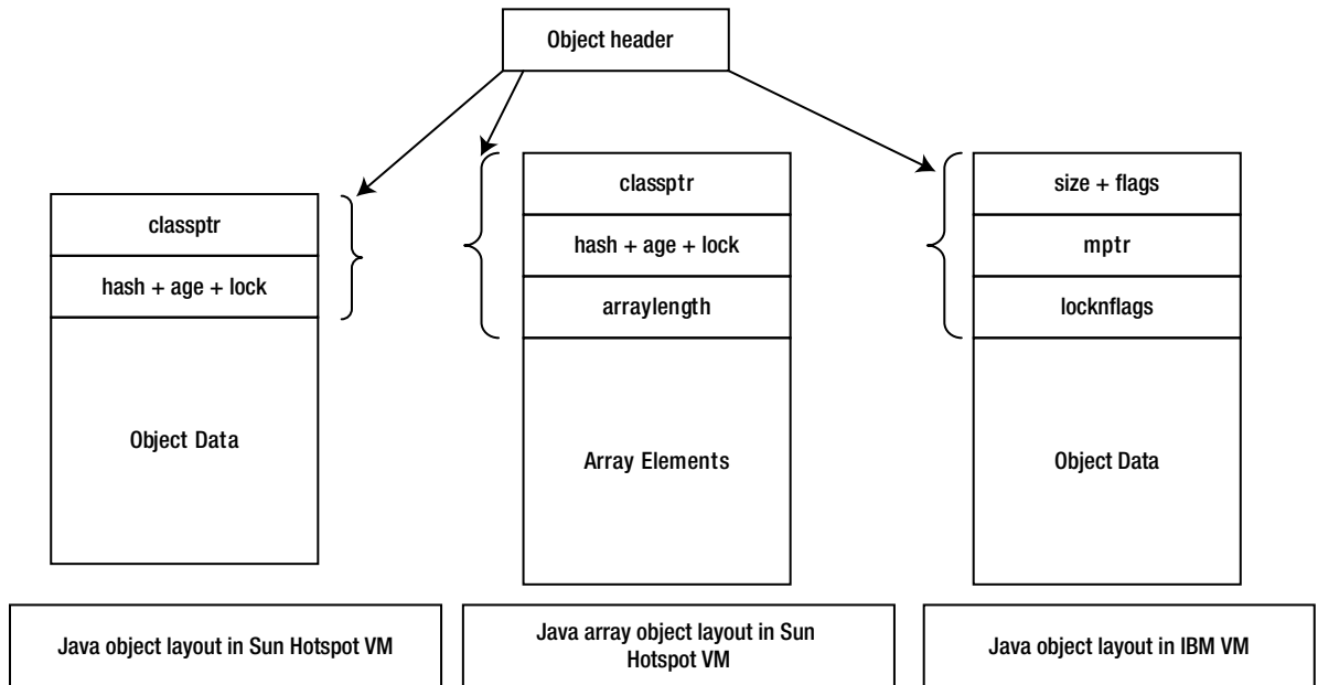
Figure 11-1. The layout of an object in the Java Hotspot VM and the IBM VM
