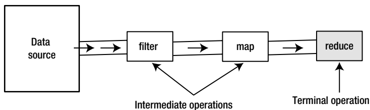
Figure 13-1. A stream pipeline
