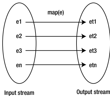
Figure 13-7. A pictorial view of the map operation
