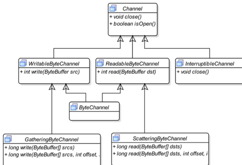
Figure 9-15. A class diagram for the channel interface
