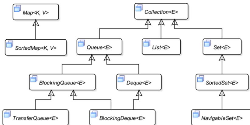
Figure 12-2. A class diagram including most interfaces in the Collections Framework
