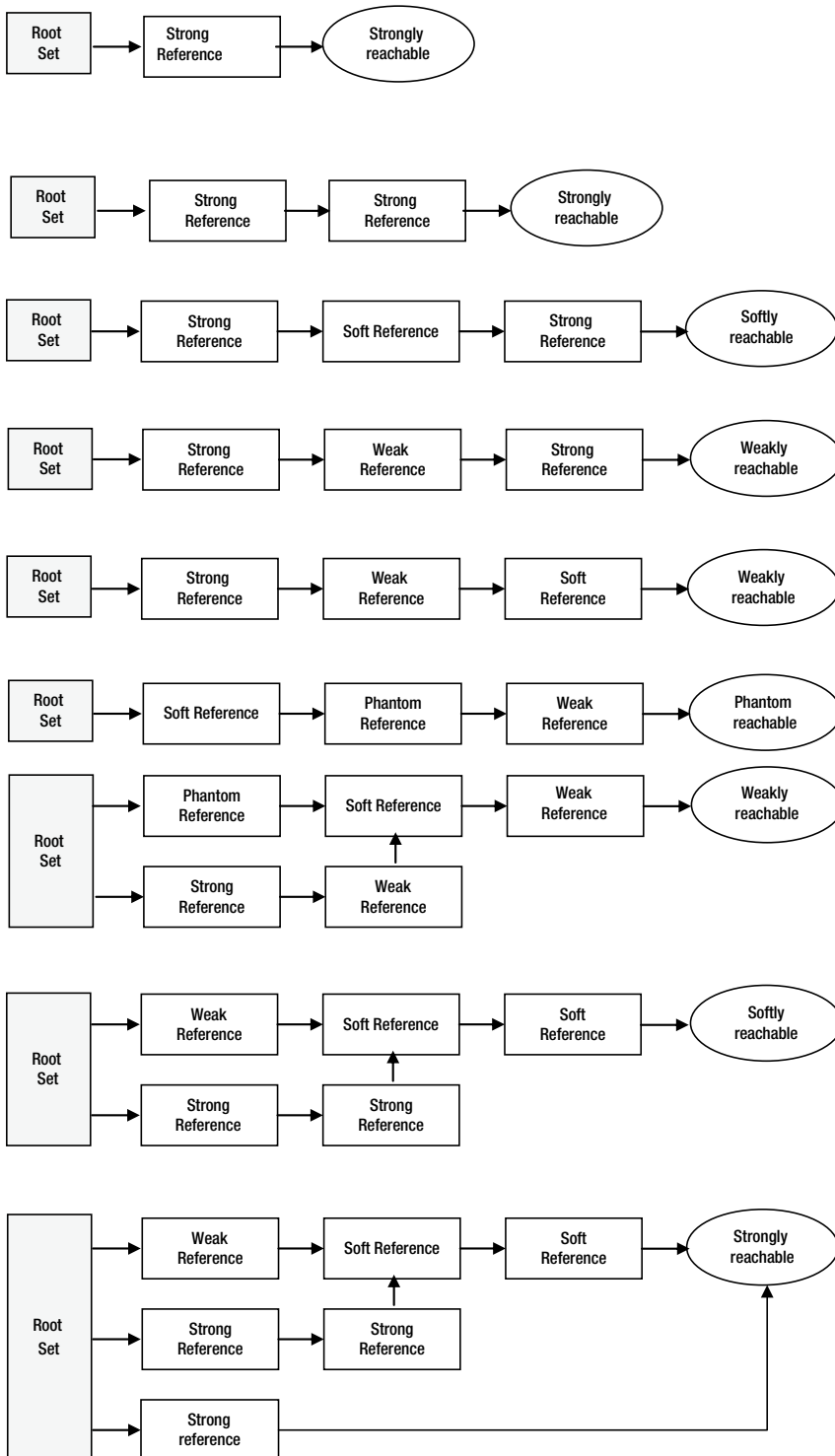
Figure 11-5. Different kinds of an object's reachability
