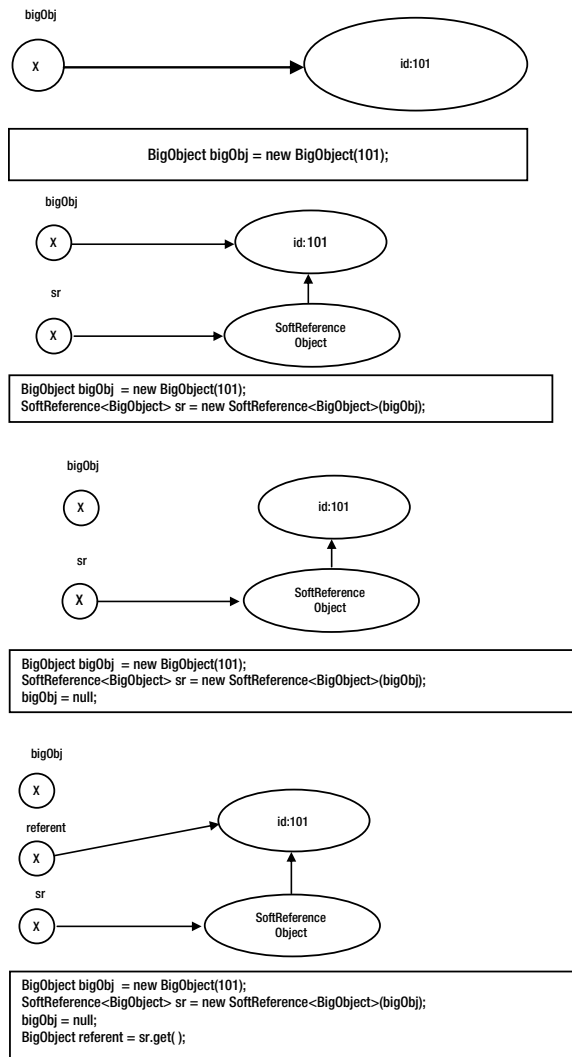
Figure 11-6. Accessing the referent of a reference object
