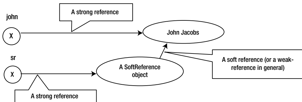
Figure 11-4. An example of a soft reference
