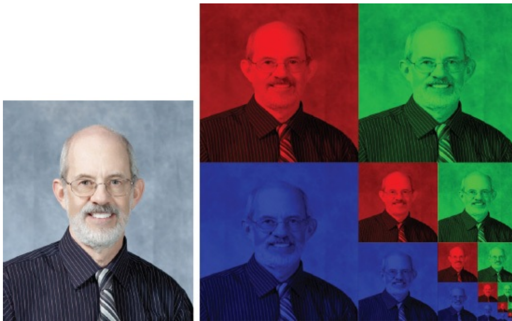
Figure 5.10 Mipmapping an image.
