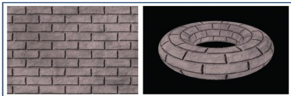
Figure 6.12 Procedurally-generated torus.
