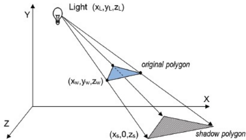
Figure 8.3 Projective shadow.
