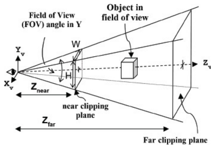
Figure 3.15 Perspective view volume or frustum.
