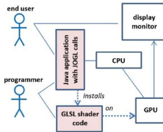
Figure 2.1 Overview of a JOGL-based graphics application.
