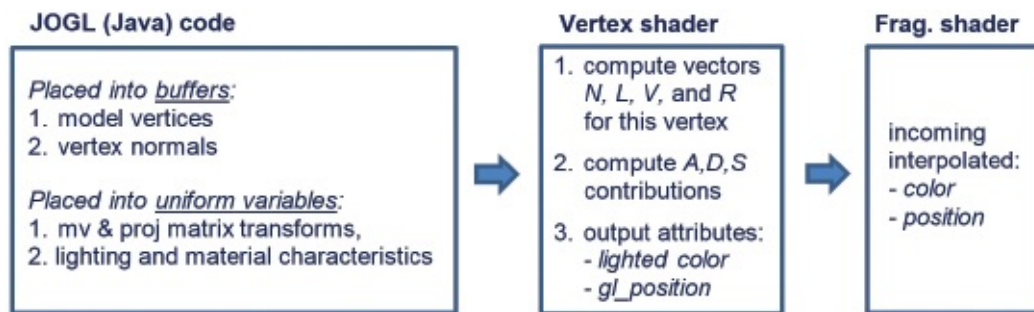
Figure 7.8 Implementing Gouraud shading.
