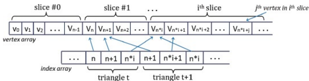
Figure 6.7 Vertex array and corresponding index array.
