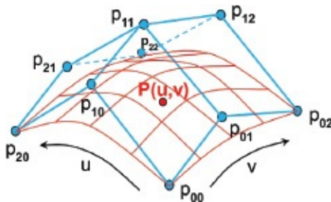
Figure 11.9 Quadratic Bézier control mesh and corresponding surface.
