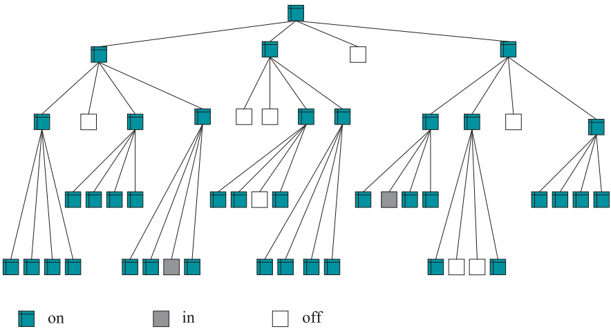
Fig. 6.8 The quadtree for Fig. 6.7
