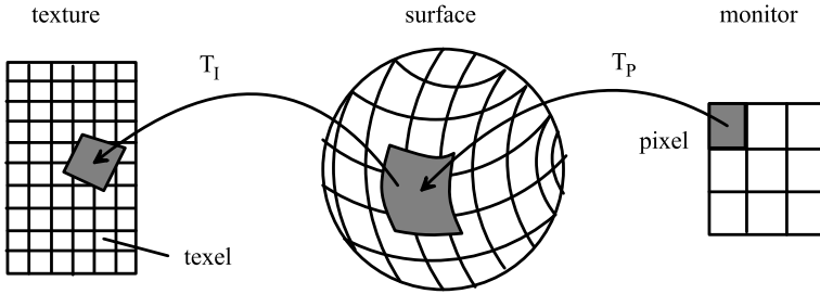
Fig. 8.16 Using a texture
