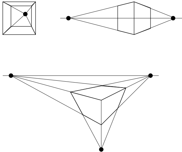
Fig. 5.12 One-, two- and three-point perspective projections
