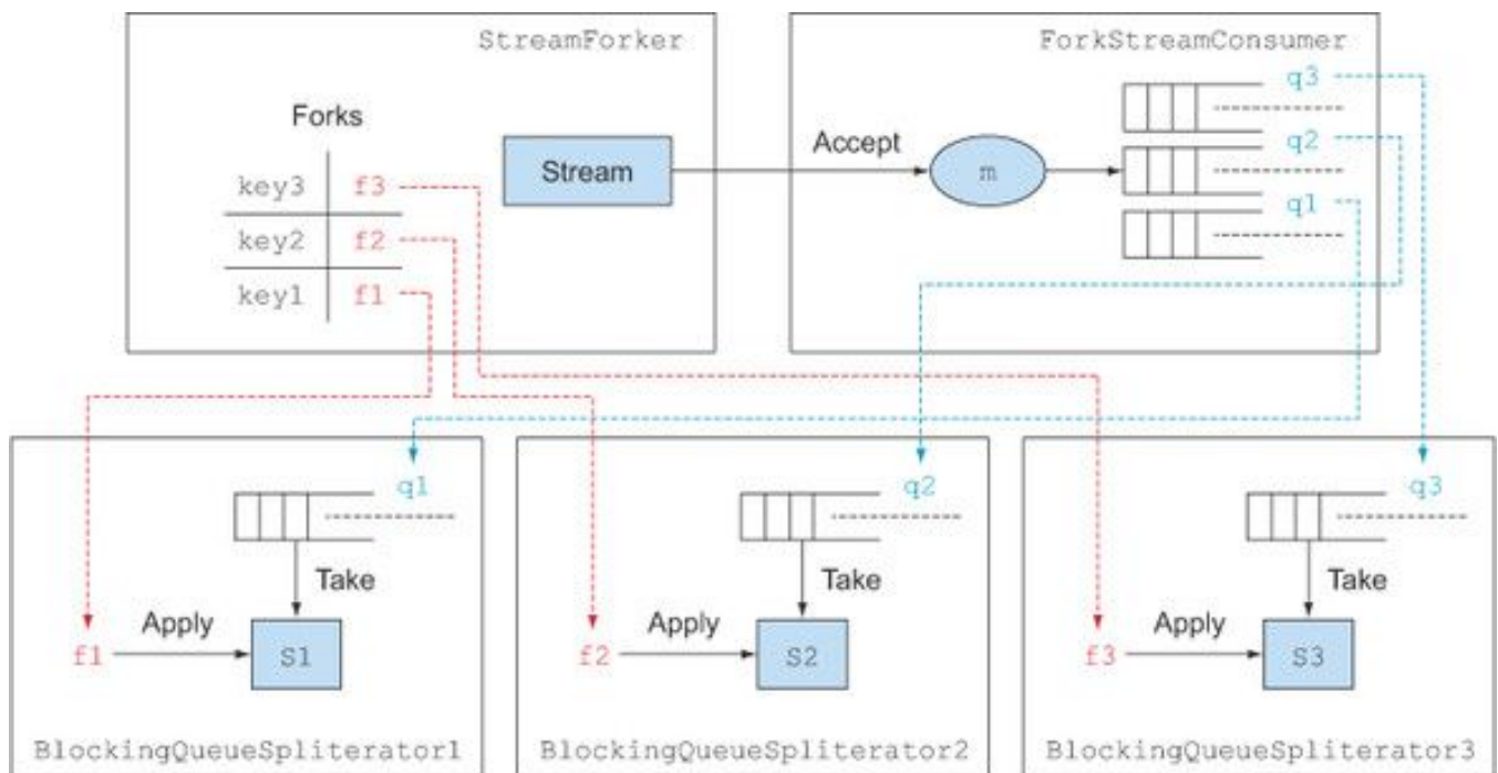
Figure C.2. The StreamForker building blocks
