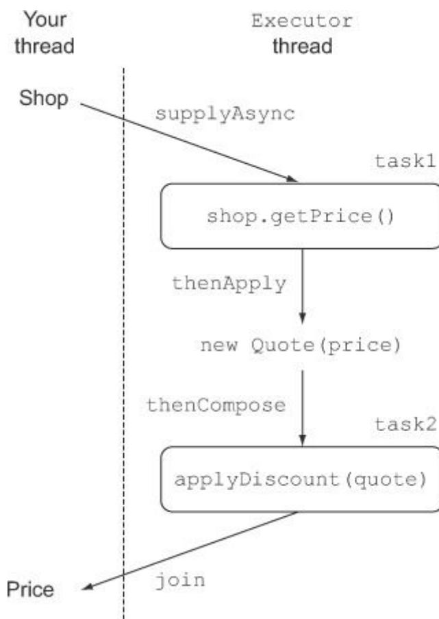
Figure 11.5. Composing synchronous operations and asynchronous tasks
