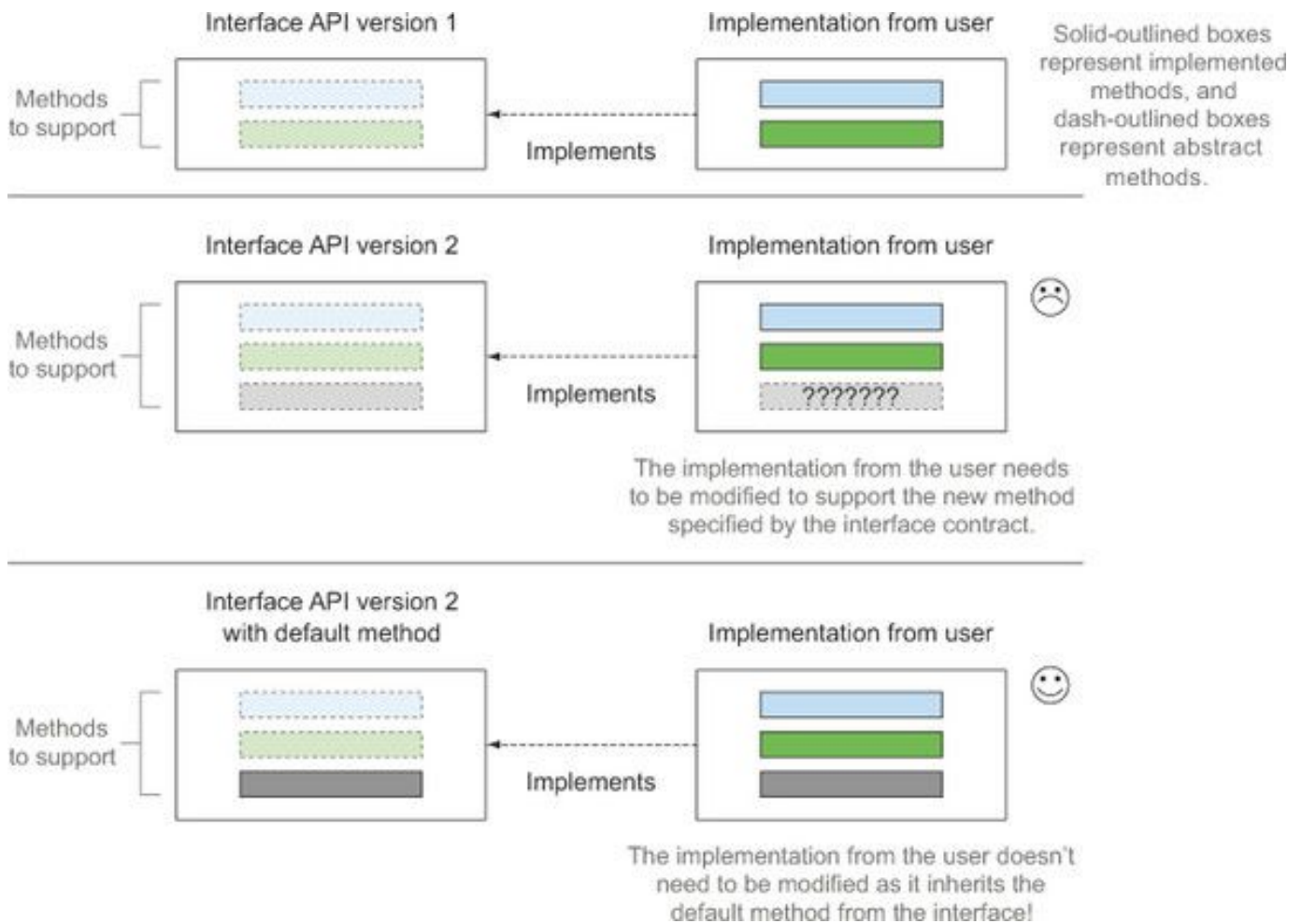
Figure 9.1. Adding a method to an interface
