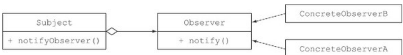
Figure 8.2. The observer design pattern
