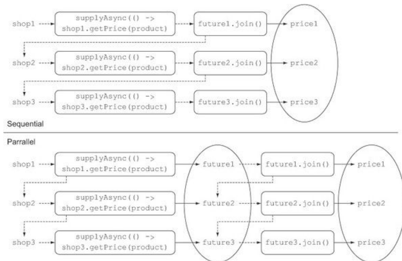
Figure 11.4. Why Stream's laziness causes a sequential computation and how to avoid it
