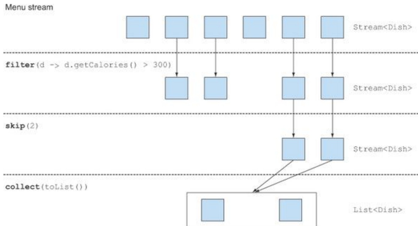
Figure 5.4. Skipping elements in a stream
