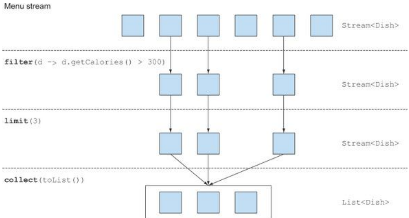
Figure 5.3. Truncating a stream
