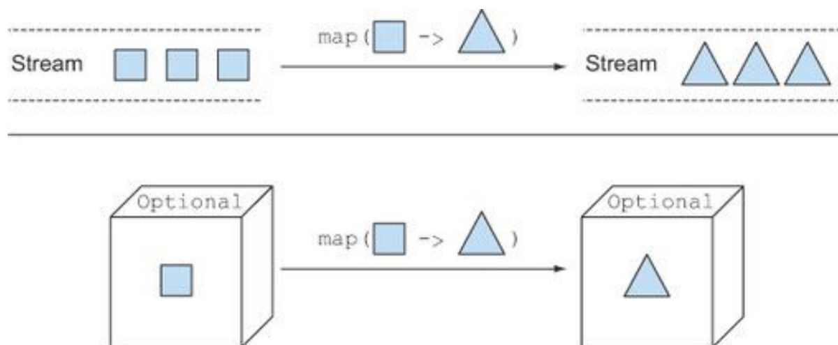
Figure 10.2. Comparing the map methods of Streams and Optionals
