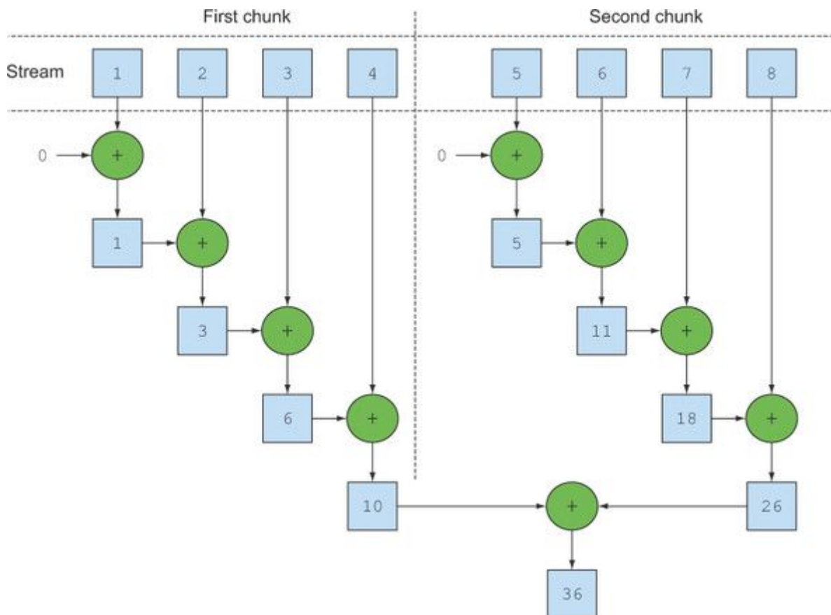
Figure 7.1. A parallel reduction operation
