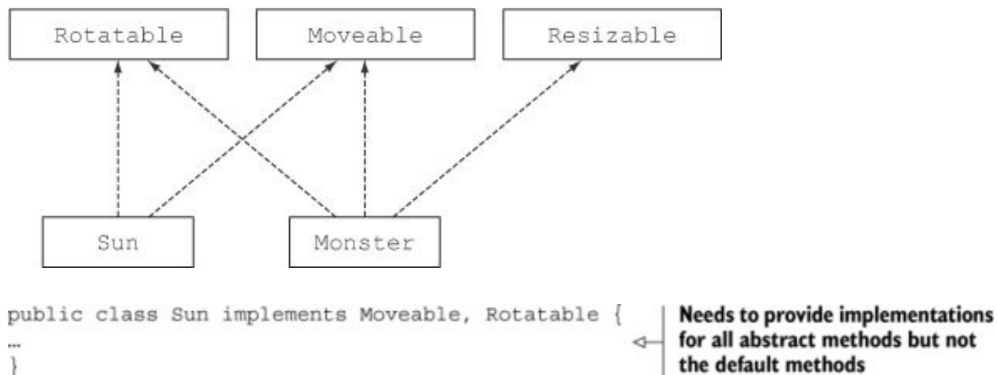
Figure 9.4. Multiple behavior composition
