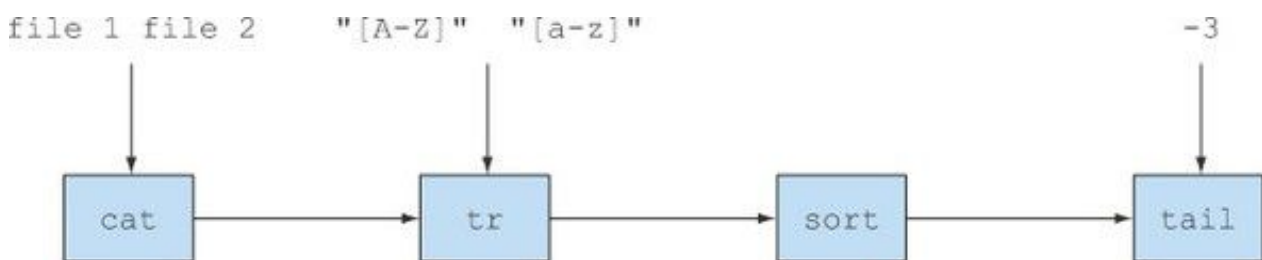
Figure 1.2. Unix commands operating on streams
