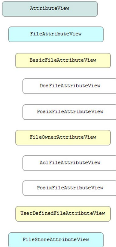
Figure 12-2. Relating view types; subtypes are indented to the right
