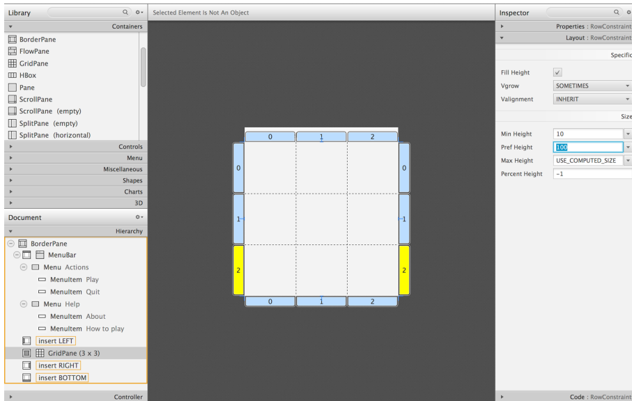
FIGURE 19-12: The BorderLayout with the menu bar and the 3x3 grid
