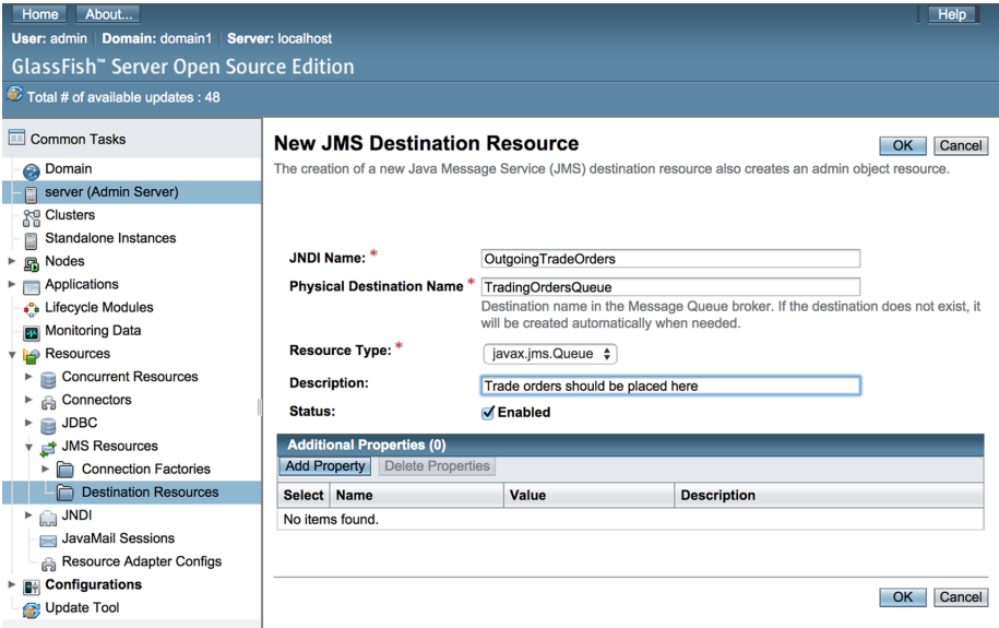
FIGURE 30-8: Mapping JNDI name to a physical queue
