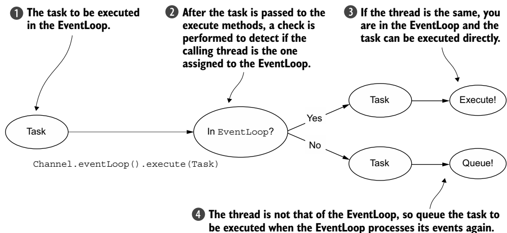
Figure 7.3 EventLoop execution logic
