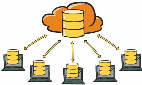
Figure 14.3 Firebase architecture
