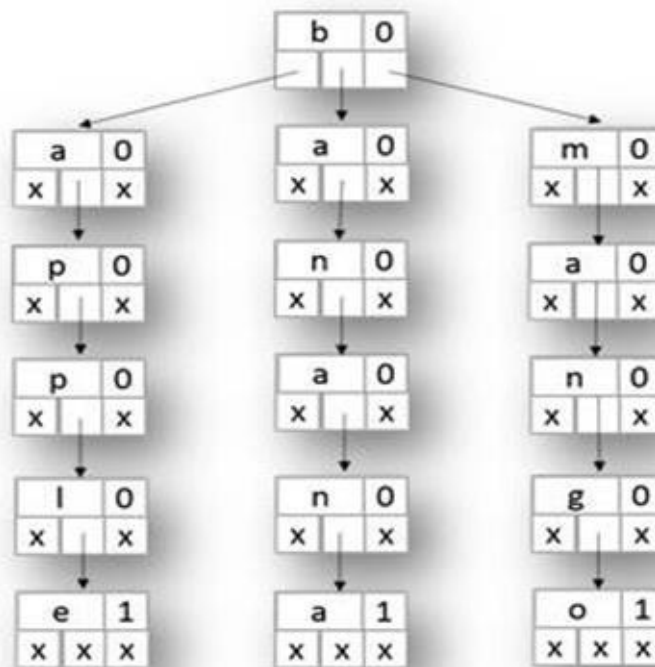
TERNARY Search Tree
