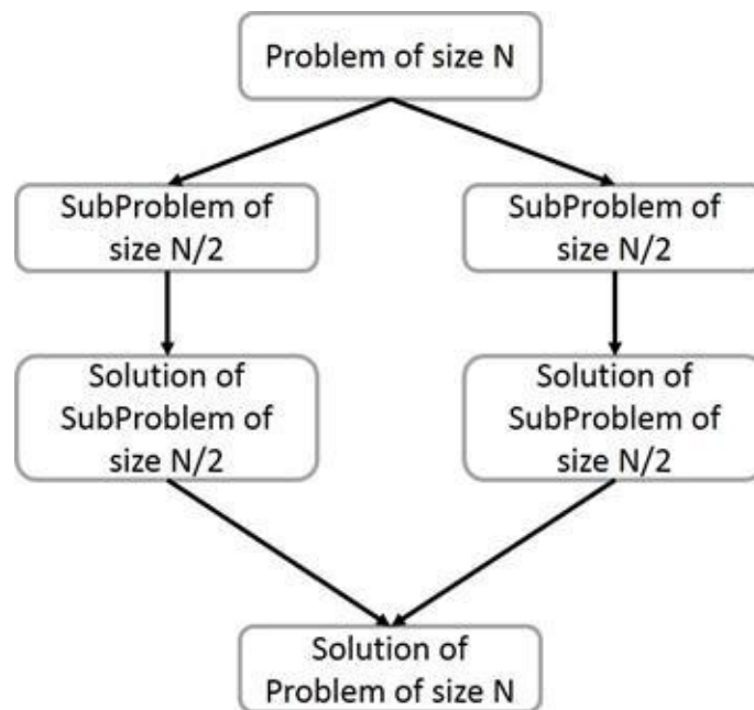
Divide-and-Conquer algorithms
