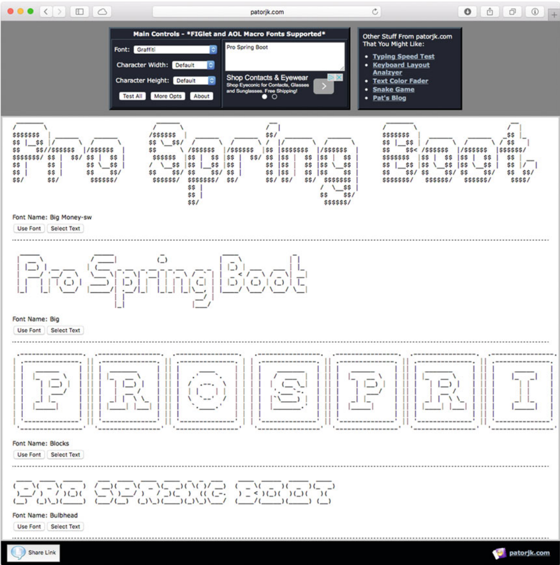
Figure 3-3. ASCII art
