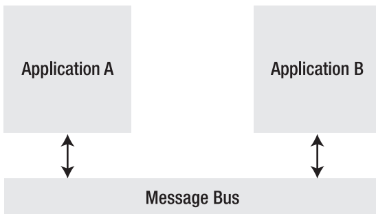
Figure 1–5. Messaging Approach
