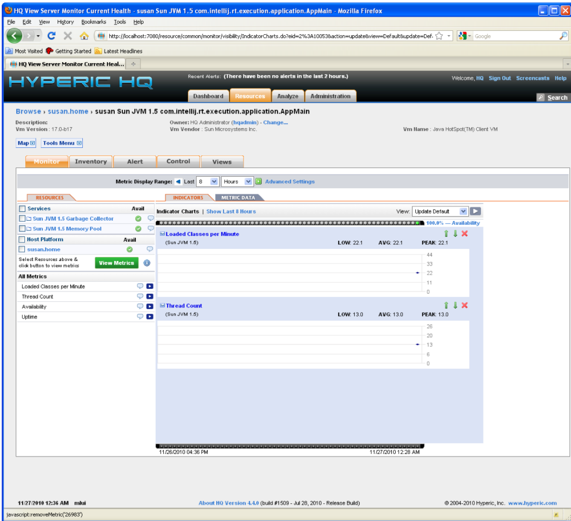
Figure 10–10. Hyperic MBeanMmonitoring
