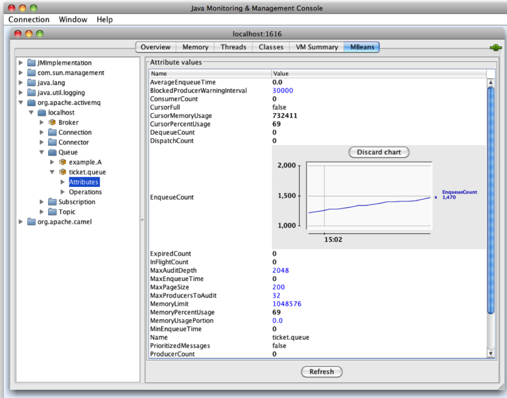
Figure 12–11. ticket.queue Attributes
