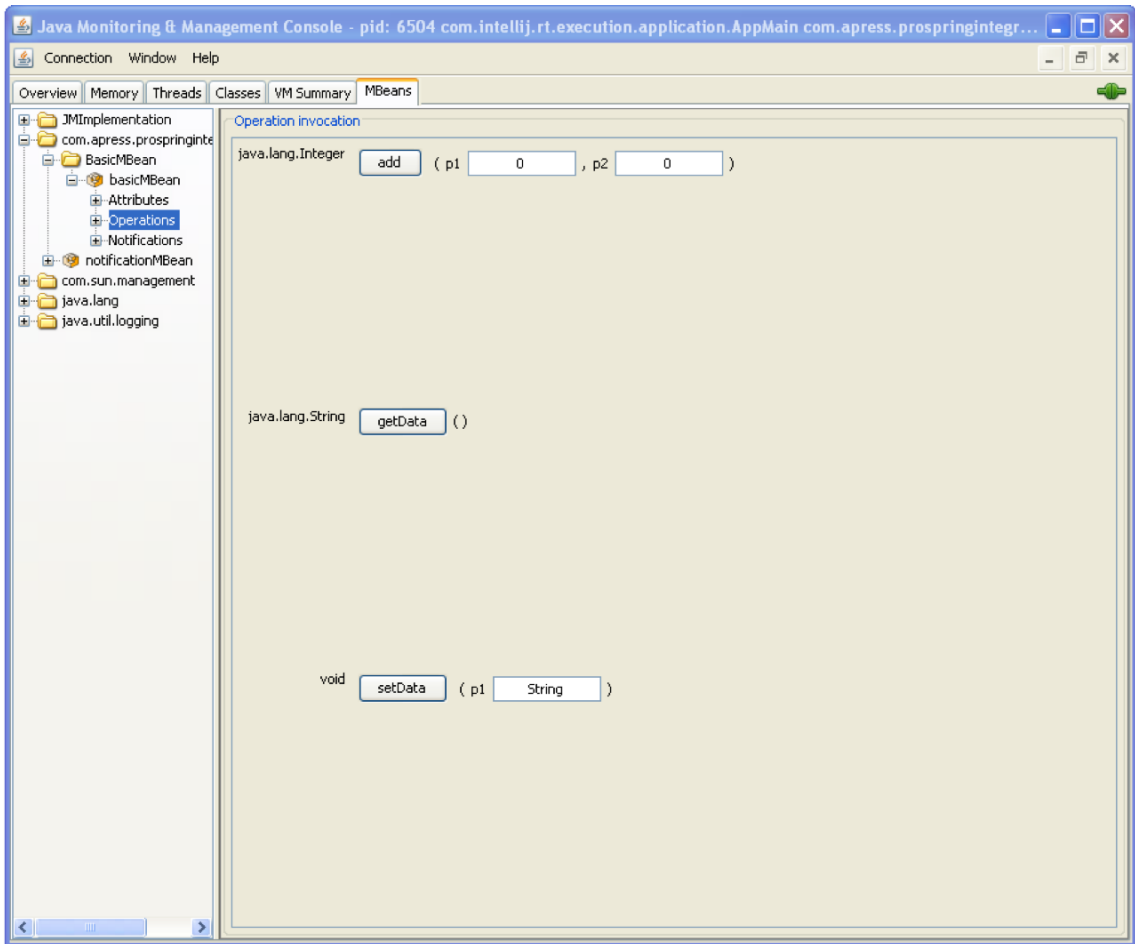
Figure 10–3. JConsole
