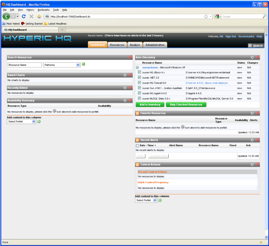
Figure 10–9. Hyperic Dashboard
