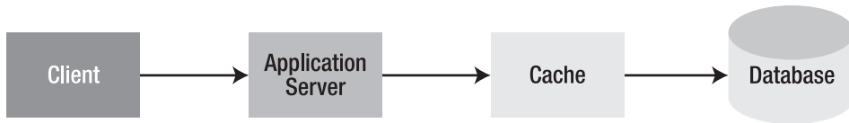
Figure 16–4. Write-behind cache
