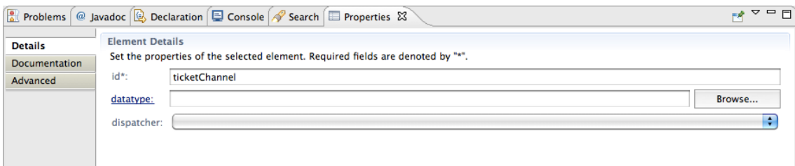
Figure 9–9. Channel Properties
