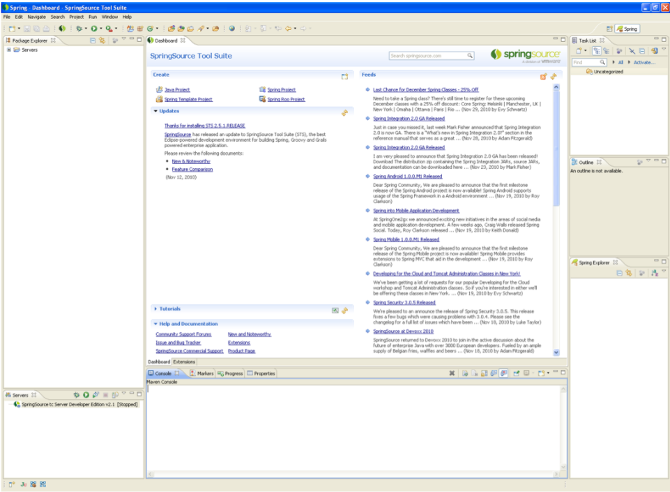
Figure 5–1. STS IDE
