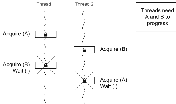
Figure 4.3 Deadlocked threads
