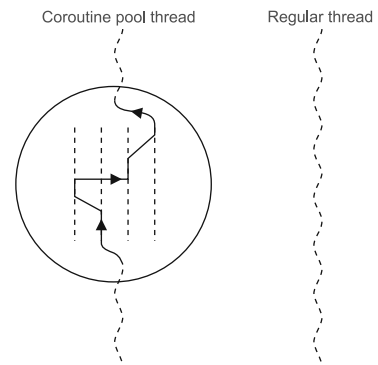
Figure 14.3 A possible coroutine model
