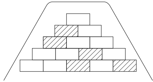
Figure 6.10 How G1 divides up the heap
