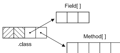
Figure 5.2 Class object and Method references
