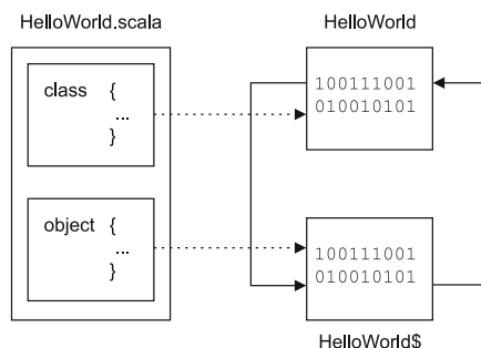
Figure 9.3 Scala singleton objects
