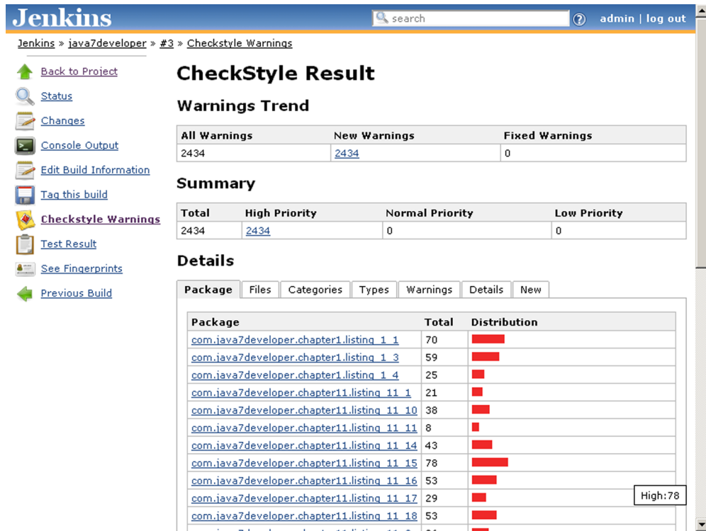
Figure 12.13 Checkstyle report
