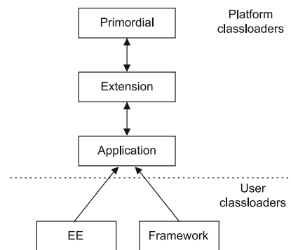
Figure 5.3 Classloader hierarchy
