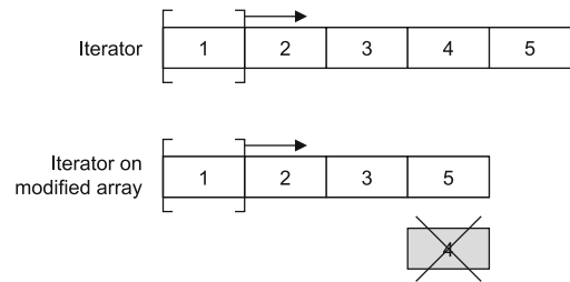
Figure 4.8 Copy-on-write array
