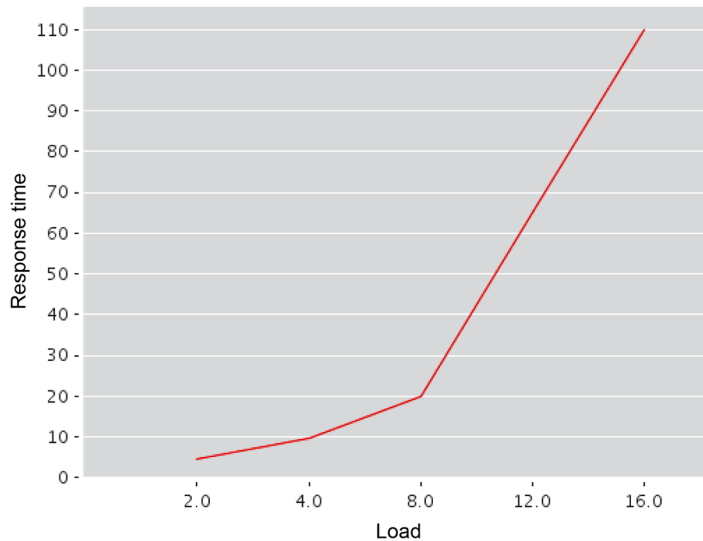
Figure 6.1 A performance elbow
