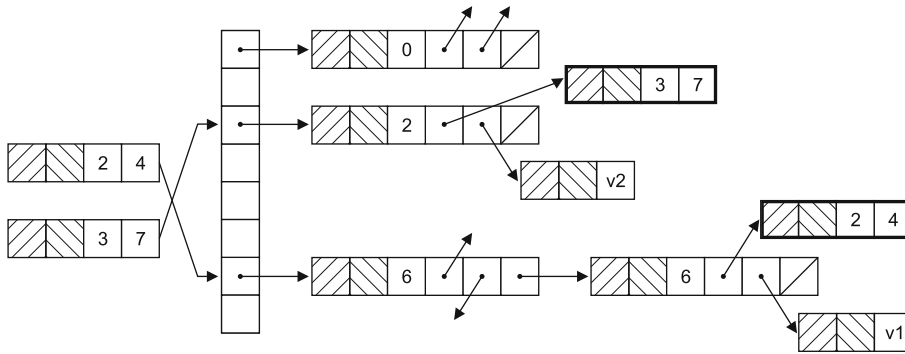
Figure 4.7 The classic view of a HashMap
