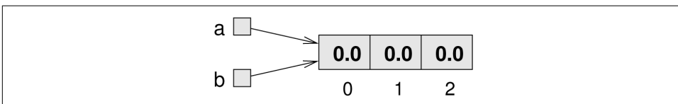
Figure 8-3. State diagram showing two variables that refer to the same array.
