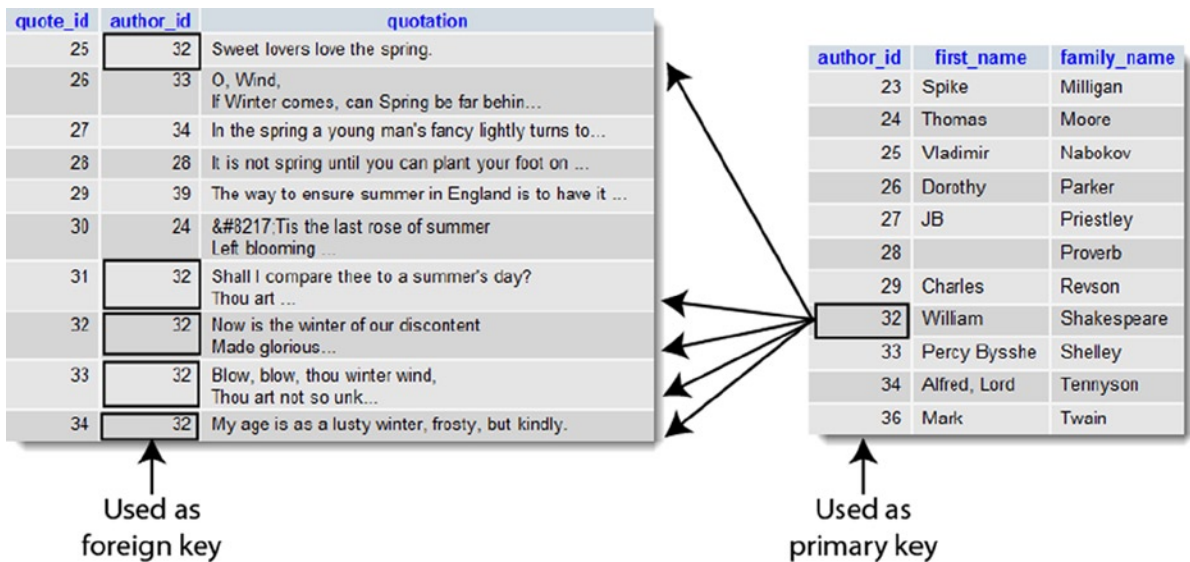
Figure 10-3. Foreign keys are used to link information stored in separate tables
