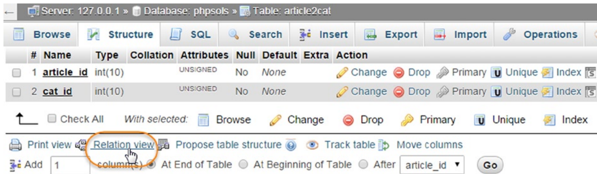
Figure 16-11. Foreign-key constraints are defined in phpMyAdmin's Relation view
