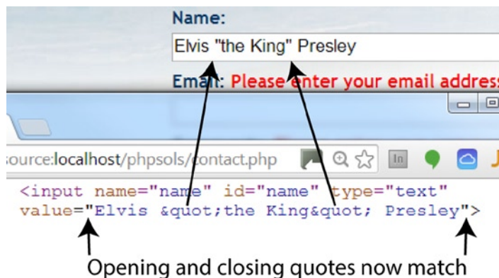
Figure 5-5. Passing the value to htmlspecialchars() before it's displayed solves the problem
