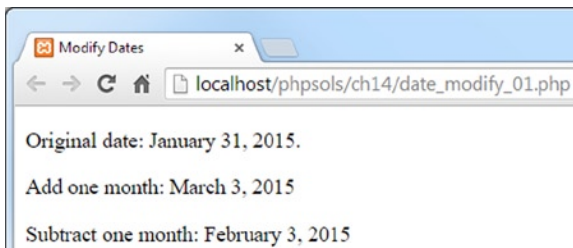
Figure 14-9. Adding and subtracting months can lead to unexpected results
