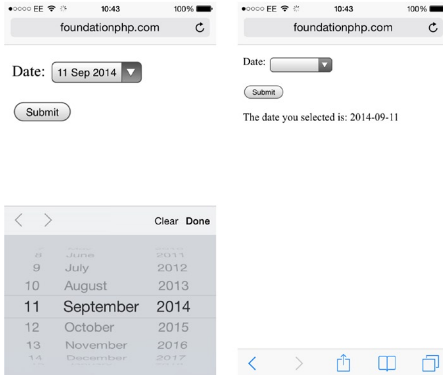
Figure 14-5. HTML5 date input fields display dates in local format, but submit them in the ISO format
