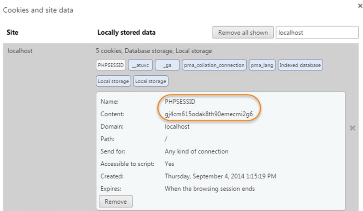
Figure 9-1. PHP sessions store a unique identifier as a cookie in the browser
