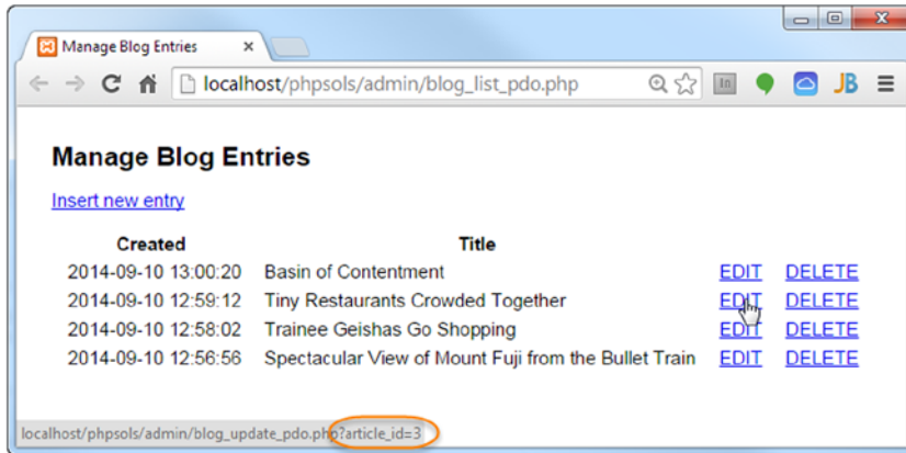
Figure 13-2. The EDIT and DELETE links contain the record's primary key in a query string
