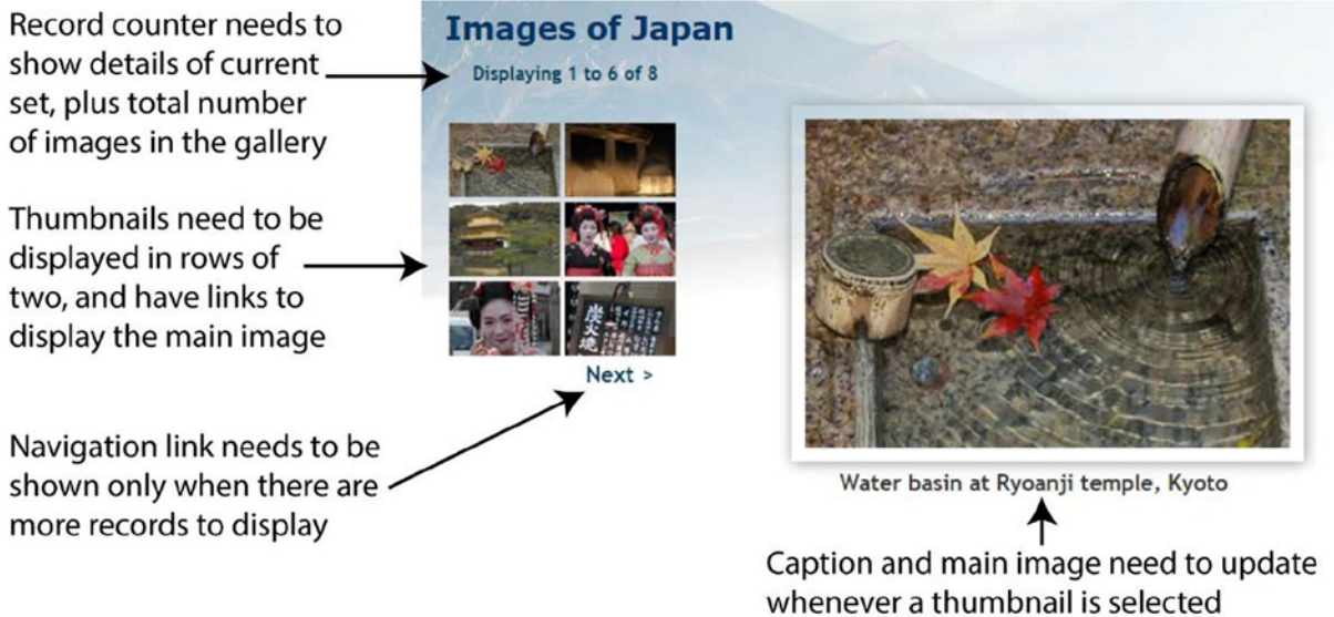
Figure 12-2. Working out what needs to be done to convert a static gallery to a dynamic one
