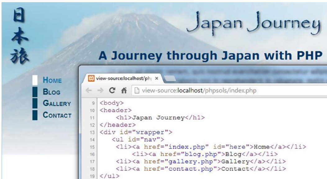
Figure 4-3. There's no output from the PHP code, so only the HTML is sent to the browser
