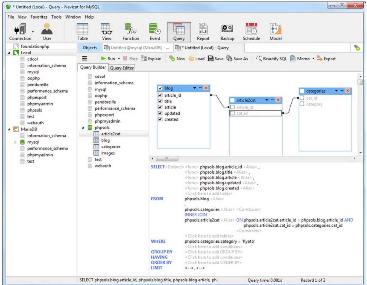
Figure 10-5. Navicat is one of the most popular graphical UIs for MySQL
