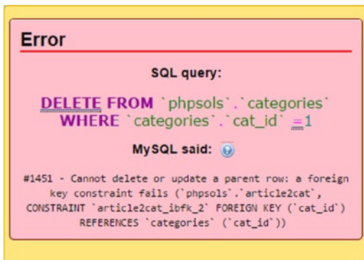
Figure 16-14. The foreign-key constraint prevents the deletion if dependent records exist
