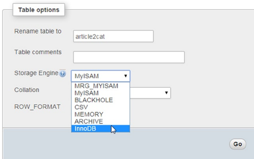
Figure 16-10. Changing a table’s storage engine is very easy in phpMyAdmin
