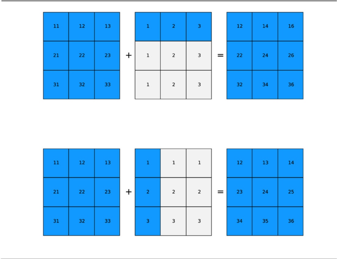
Figure 2-2. Visualization of broadcasting of row and column vectors into the shape of a matrix. The highlighted elements represent true elements of the arrays, while the light gray shaded elements describe the broadcasting of the elements of the array of smaller size
