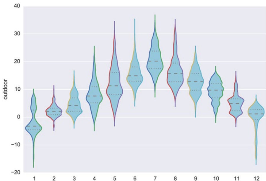
Figure 12-11. Violin plot for the outdoor temperature grouped by month
