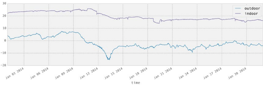
Figure 12-4. Plot of the time series for indoors and outdoors temperatures for a selected month (January)
