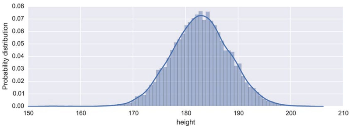
Figure 16-8. Probability distribution for prediction of height for weight being 90 kg
