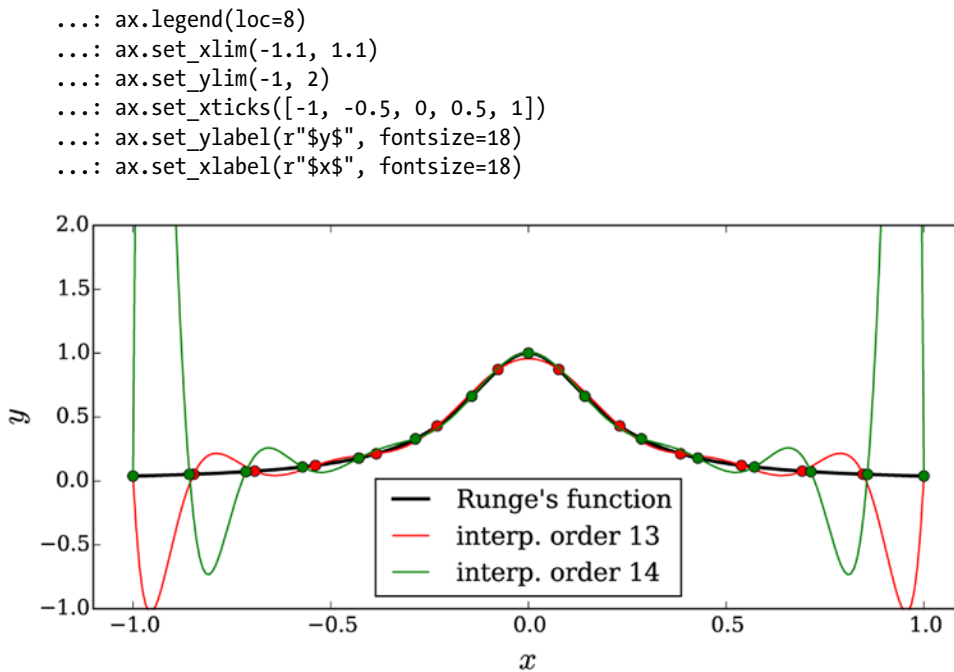
Figure 7-2. The Runge function together with two high-order polynomial interpolations
