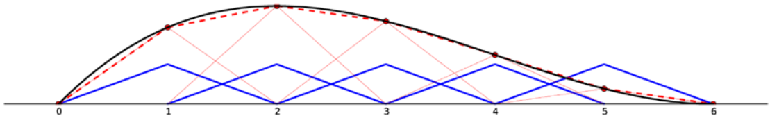
Figure 11-3. An example of possible basis functions (blue lines), with local support, for the one-dimensional domain [0, 6]
