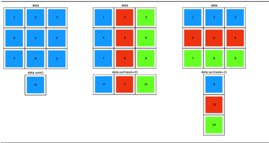
Figure 2-3. Illustration of array aggregation functions along all axes (left), first axis (center), and the second axis (right) of a two-dimensional array of shape 3 \times 3
