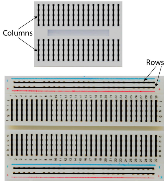
Figure 9—How sockets on a breadboard are connected
