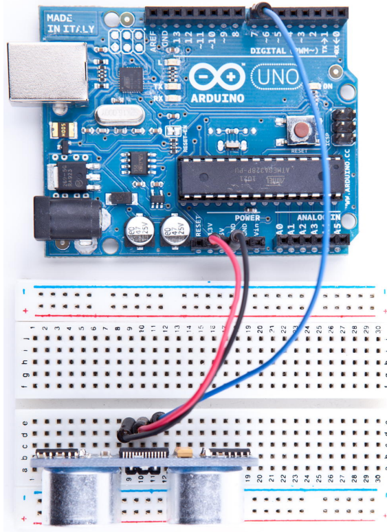
Figure 16—Photo of PING))) basic circuit
