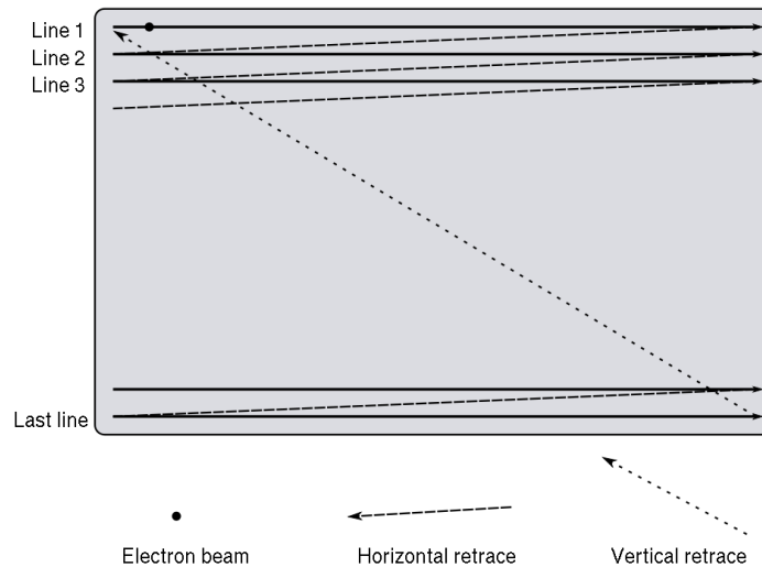
Figure 23—How raster scan works
