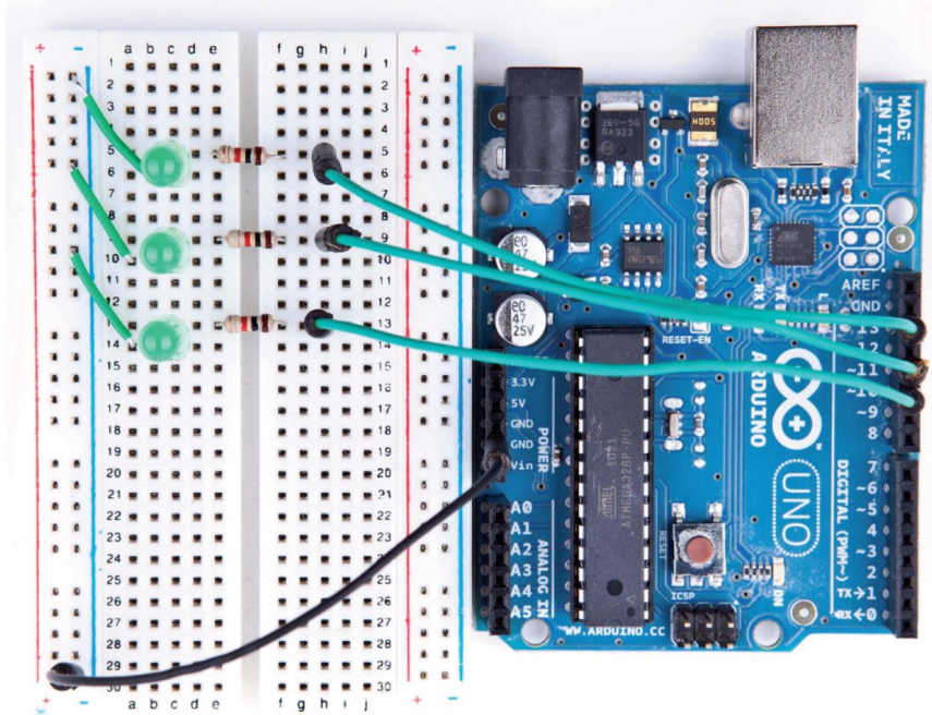
Figure 11—A first working version of our binary die
