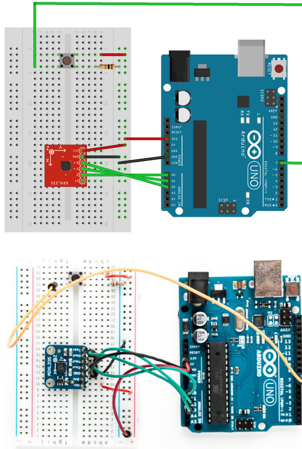
Figure 19—Game controller with accelerometer and pushbutton
