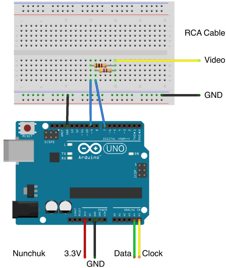
Figure 27—Circuit of our video game console
