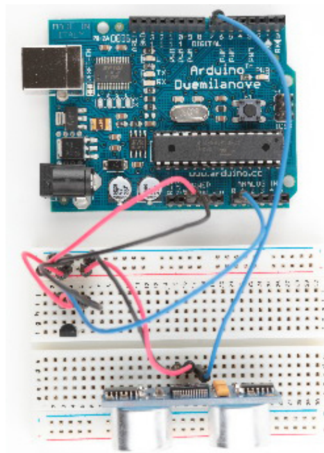
Figure 18—Photo of final circuit
