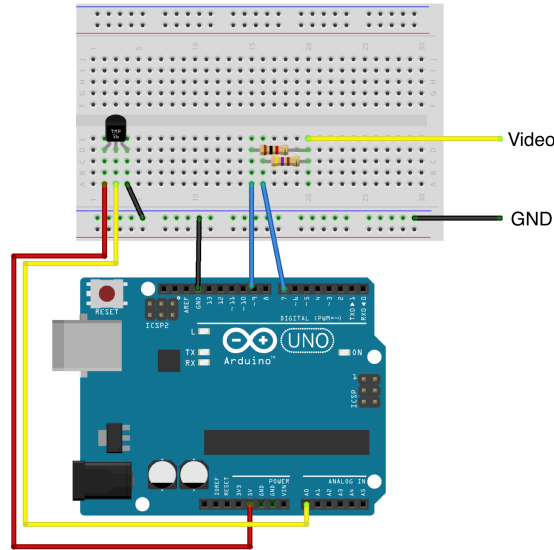
Figure 24—Circuit of the TV thermometer
