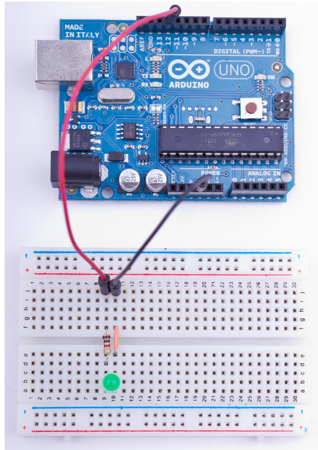
Figure 10—Connecting an LED on a breadboard to the Arduino
