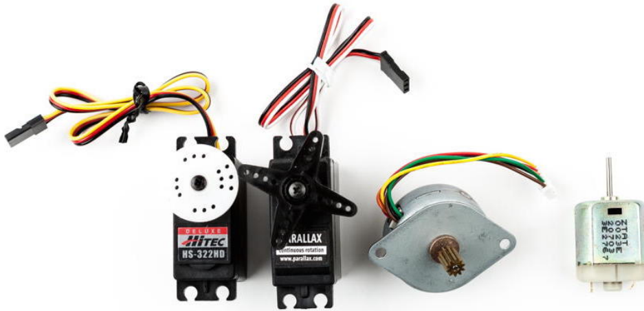
Figure 31—Motor types from left to right: standard servo, continuous rotation servo, stepper, DC motor
