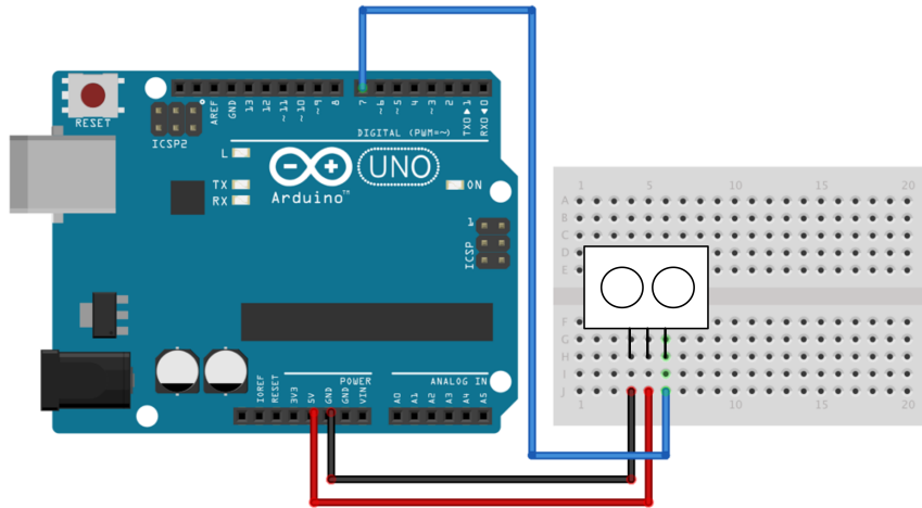
Figure 15—PING))) basic circuit
