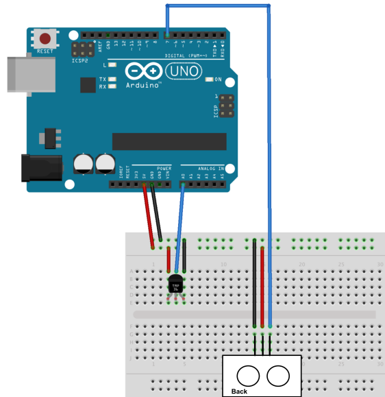
Figure 17—The TMP36 and the PING))) sensors working together
