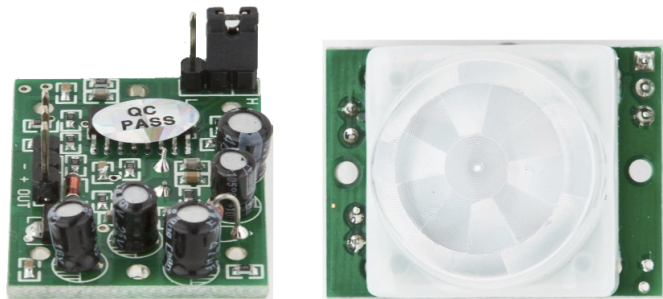
Figure 29—Top and bottom of a passive infrared sensor
